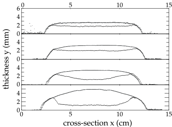
FIG. 16: Flow and deposit morphologies for an increasing polydispersity degree, from top to bottom: batches 2, 3, 4, and 8 (see table I for size distributions) (flux: 8.15 \text{ g/s} , roughness: 425\text{-}600 \mu\text{m} , slope: 25^\circ ).
