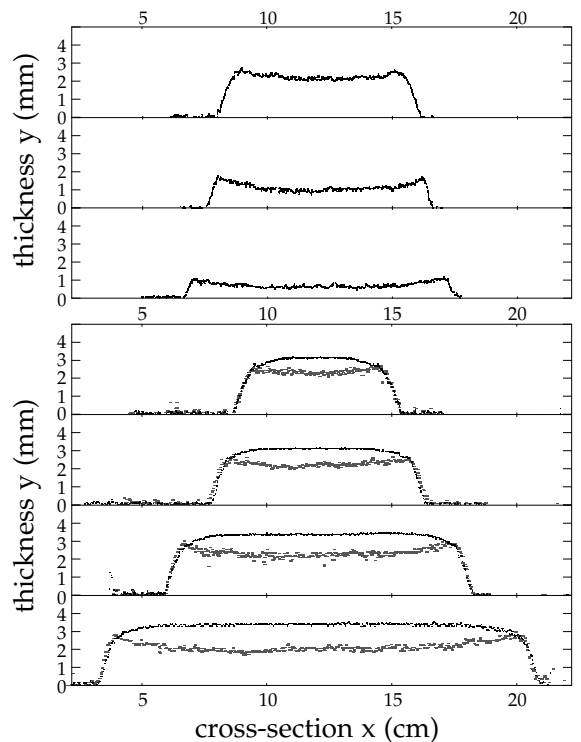
FIG. 8: (top) Increasing the angle of the slope enhances the morphology of the deposit. From top to bottom: 25^\circ , 27^\circ , and 29^\circ (flux: 7.1 g/s). (bottom) Evolution of the morphology of a flow and its deposit for different fluxes, from top to bottom: 3.7, 8, 17.5, and 38 g/s (slope: 25^\circ ). The width of the levées varies slightly, although the width of the deposit varies a lot (beads: 300-400 \mu\text{m} , roughness: 425-600 \mu\text{m} ).
