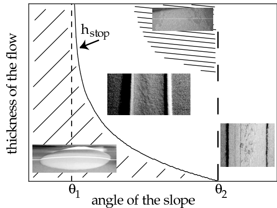
FIG. 12: Location of the deposit types, shown by the inset photographs, compared to the h_{stop}(\theta) curve. For flow conditions below the curve, the deposit has a rounded shape. The levée/channel morphology exists above the curve except when instabilities occur (high angle and thickness). ‘Levées with an empty channel’ can be observed for angles slightly above \theta_2 (dark beads for this inset). For higher angles, there is no deposit either in the levées, or in the channel. Consequently, the levée/channel morphology, with some matter remaining in the channel, occurs only between the \theta_1 and \theta_2 angles.
