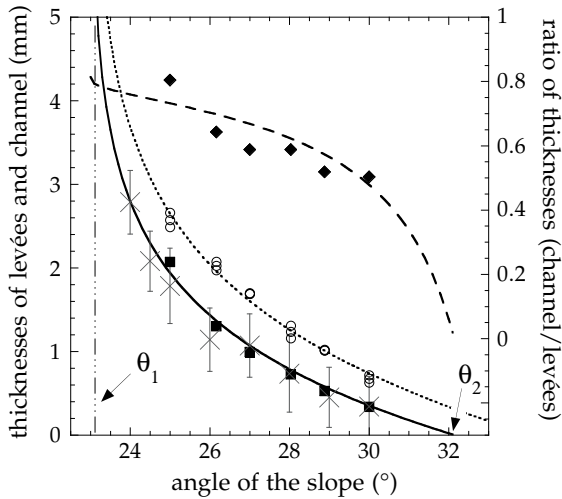
FIG. 9: Thickness of deposit: (O) h_{levée} , and (■) h_{channel} . Fits come from equation (1) with the same values of \theta_1 and \theta_2 according to: (—) “ h_{stop} curve”, and (---) “ h_{stop} + constant ” curve. (◆) the h_{channel}/h_{levée} ratio and (- -) the fit obtained from the ratio of both fits show the decrease observed in the field. (×) Thickness of the deposit of wide laterally confined flows, with error bars. Thicknesses of the deposit of both an unconfined flow, and a confined flow are equal (flux: 7 g/s for confined flows, and large enough to cover the whole plane for confined flows, beads: 300-400 \mu\text{m} , roughness: 425-600 \mu\text{m} ).
