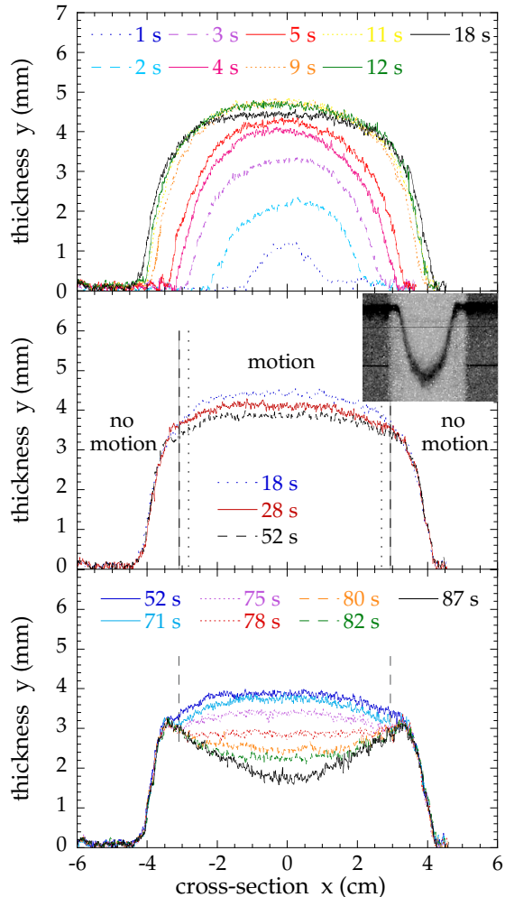
FIG. 4: (top) Arrival of the front of the flow at the chosen location: both height and width increase with time. X-axis is taken perpendicularly to the flow direction. (middle) Stable flow with constant width. The slight decrease of the height corresponds to a longitudinal convex shape of the front. The two lines limit the area where there is a surface motion: lateral static zones exist on each border of the flow (slightly wider at 18 s). Inset: a line of dark particles poured instantaneously on the surface of the flow shows the two static lateral borders and the surface velocity profile. (bottom) After stopping the supply, the central channel partly empties: the final morphology is high lateral levées with a low central channel. Here, the channel is not flat because of the ‘small’ flux used. The levées record the height reached by the flow in the lateral static zones (beads: 300-400 \mu\text{m} , roughness: 425-600 \mu\text{m} , flux: 7 g/s, slope: 25°)
