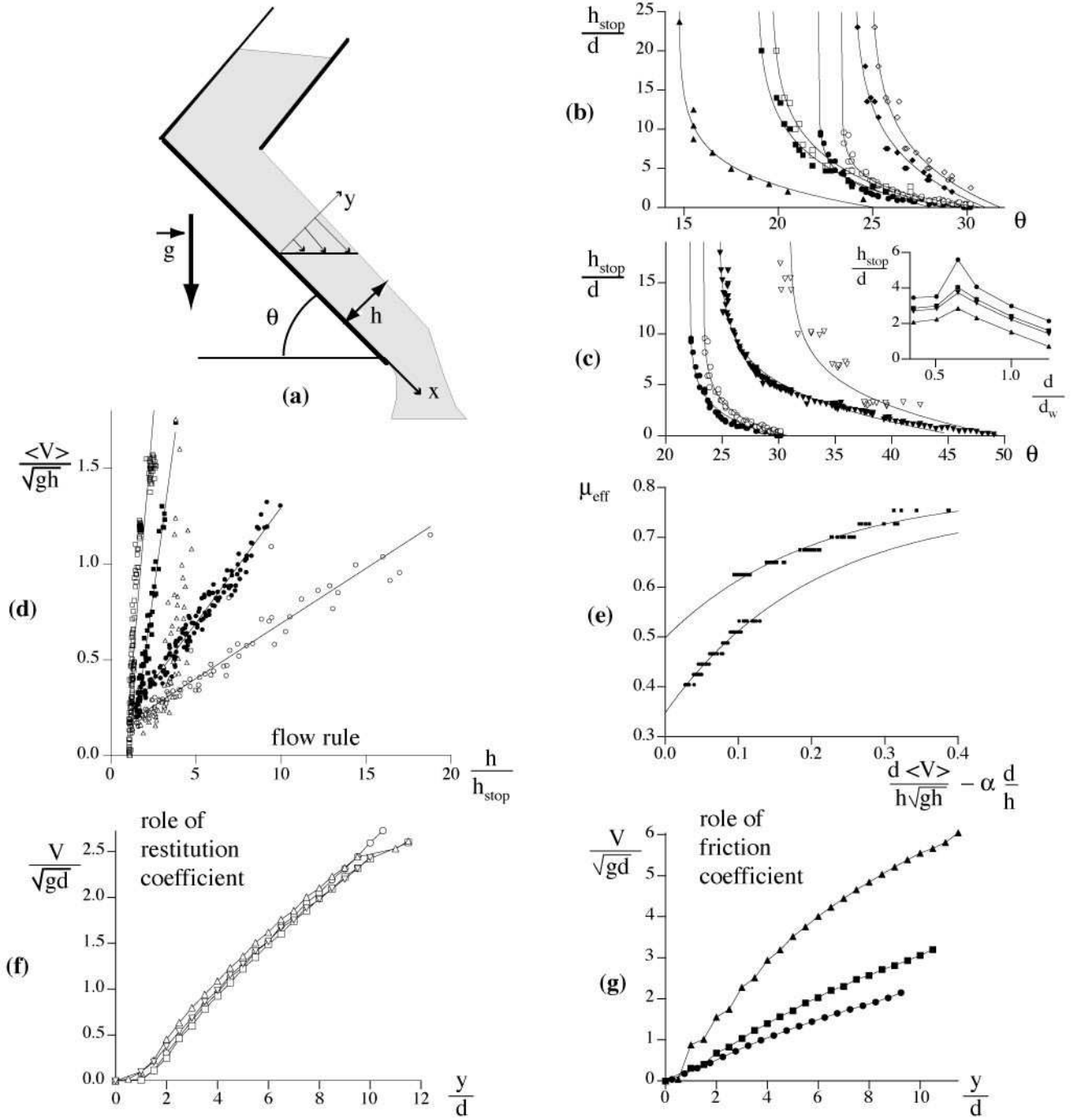
Fig. 5. Rough inclined plane. (a) Set up. (b) h_{\text{stop}}(\theta) (black symbols) and h_{\text{start}}(\theta) (white symbols) from simulations IP3 ( \blacktriangle ), experiments IP5 with glass beads ( \circ, \bullet ), IP6 with mustard seeds ( \diamond, \blacklozenge ) or with glass beads on carpet ( \square, \blacksquare ). See text for the fit. (c) Same as (b) for experiments IP5 with glass beads ( \circ, \bullet ), IP7 with glass beads on velvet ( \nabla, \blacktriangledown ). Inset: h_{\text{stop}} for different roughness condition from experiment IP8 \theta = 27^\circ ( \bullet ), \theta = 28^\circ ( \blacksquare ), \theta = 28.3^\circ ( \blacktriangledown ), \theta = 30^\circ ( \blacktriangle ). (d) Froude number \langle V \rangle / \sqrt{gh} as a function of h/h_{\text{stop}}(\theta) from simulation IP3 ( \circ ), experiments IP5 with glass beads on glass beads ( \bullet ), sand on sand ( \square ), IP6 sand on moquet ( \blacksquare ), IP7 glass beads on velvet ( \triangle ). Lines are fits by eq. (7). (e) Effective friction deduced from the flow rule (see text). Experiment IP5 with glass beads ( \bullet ), with sand ( \blacksquare ). Continuous lines are deduced from eq. (8) and fit of h_{\text{stop}}(\theta) . (f) Velocity profiles from simulations IP4 ( \theta = 14.4^\circ , \mu = 0 ) for different restitution coefficients e = 0.4 ( \triangle ), e = 0.6 ( \nabla ), e = 0.7 ( \square ) and e = 0.8 ( \circ ). (g) Velocity profiles from simulations IP4 ( \theta = 18^\circ , e = 0.6 ) for different friction coefficients \mu = 0 ( \triangle ), \mu = 0.25 ( \blacksquare ) and \mu = 0.5 ( \bullet ).
