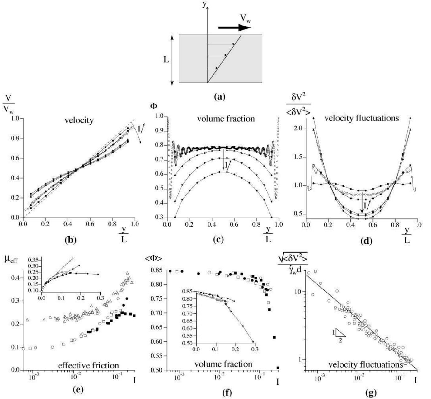
Fig. 2. Plane shear. (a) Setup. (b) Velocity profiles rescaled by the wall velocity from simulations PS1: I between 0.2 and 0.5 ( e = 0.8 ) (black symbols) and PS2: I = 0.23 ( e = 0.1 , \mu_p = 0.4 ) ( \circ ). (c) Volume fraction profiles as a function of I from simulations PS1: I between 0.2 and 0.5 ( e = 0.8 ) (black symbols) and PS2: I = 0.23 ( e = 0.1 , \mu_p = 0.4 ) ( \circ ). (d) Velocity fluctuations profile normalised by its mean value across the cell as a function of I from simulations PS1: I between 0.06 and 0.5 ( e between 0.6 and 0.98) (black symbols), and PS2: I = 0.23 ( e = 0.1 , \mu_p = 0.4 ) ( \circ ). (e) Effective friction \mu_{\text{eff}} as a function of I measured at the wall in simulation PS1: e = 0.1 ( \bullet ) and e = 0.9 ( \blacksquare ) and inside the flow in simulation PS2: e = 0.1 ( \circ ), e = 0.9 ( \square ), both for \mu_p = 0 . ( \triangle ) correspond to simulations PS2 with 0.1 < \mu_p < 0.8 . Inset: same curves in linear-linear representation. (f) Mean volume fraction \langle \Phi \rangle as a function of I from simulations PS1: e = 0.1 ( \bullet ) and 0.8 ( \blacksquare ) and PS2: e = 0.1 ( \circ ) and 0.9 ( \square ). Inset: same curves in linear-linear representation. (g) Relative velocity fluctuations as a function of I from simulations PS2: e = 0.1 and 0.9 , \mu_p = 0, 0.4 and 0.8 .
