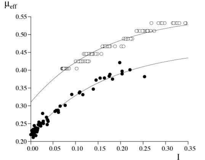
Fig. 8. Comparison of the effective friction function of I in the plane shear ( \bullet ) and the inclined plane ( \circ ) configurations.
