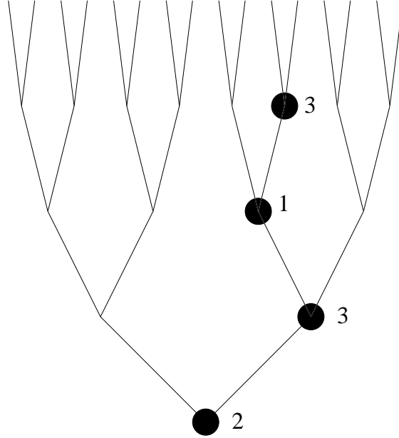
Fig. 1: A typical state of the bindweed model for s = \{1, 2, 3\} , \sigma = 2313 , and \mathbb{T} the binary tree.
