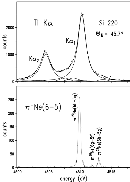
FIG. 1: Upper : Ti K\alpha doublet fitted by a sum of six Voigt functions. Lower : \pi -Ne 6 \rightarrow 5 transitions showing fine-structure and isotopic effects. Comparison of the two spectra demonstrates the energy coincidence of the Ti K\alpha_1 and of the \pi^{20}\text{Ne} 6h \rightarrow 5g lines.
