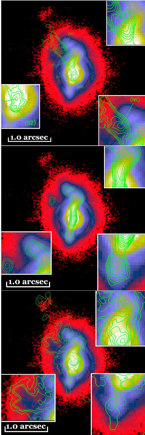
Fig. 2. On our logscale M band image are superimposed contours, from top to bottom, of : radio 5 GHz (Gallimore et al. 1996) ; 12.5 \mu\text{m} (Bock et al. 2000) ; O III line emission (Capetti et al. 1995). Various insets of magnified regions are also shown.
