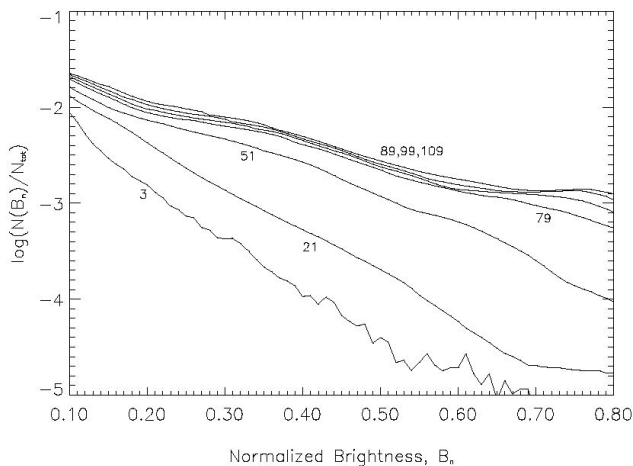
Fig. 6. Brightness histogram analysis of the H_2 \nu = 1-0 S(1) emission at 2.121 \mu\text{m} in the ESE region. Figures besides the curves shown represent the number of pixels on the square over which the data have been spatially averaged.
