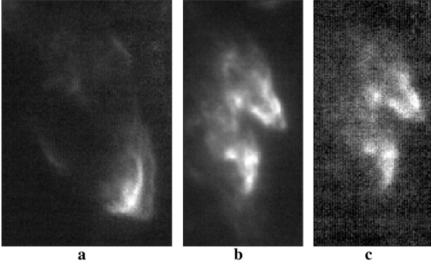
Fig. 3. a). A detailed view ( 3.5'' \times 5.0'' ) of object a (see Fig.1) in v=1-0 S(1) \text{H}_2 emission at 2.121 \mu\text{m} . b). of object b ( 2.5'' \times 5.0'' ) in the same line. c). Detail ( 2.5'' \times 5.0'' ) of object b in the 1-0 S(0) \text{H}_2 emission line at 2.22 \mu\text{m} .
