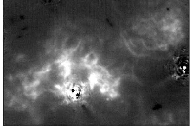
Fig. 4. A detailed view of object c (see Fig.1) in v=1-0 S(1) \text{H}_2 emission at 2.121 \mu\text{m} . Image size: 7.5'' \times 5.0'' .
