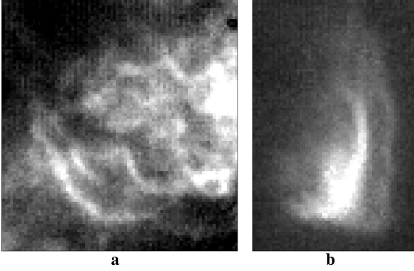
Fig. 5. a). Detail (1.56''x2.40'') of the NW part of Fig. 4 and b). of Fig. 3a (2.24''x2.40'') showing narrow filamentary structure.
