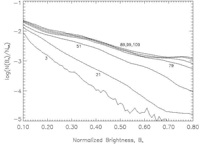
Fig. 6. Brightness histogram analysis of the \text{H}_2 v=1-0 S(1) emission at 2.121 \mu\text{m} in the ESE region. Figures besides the curves shown represent the number of pixels on the square over which the data have been spatially averaged.
