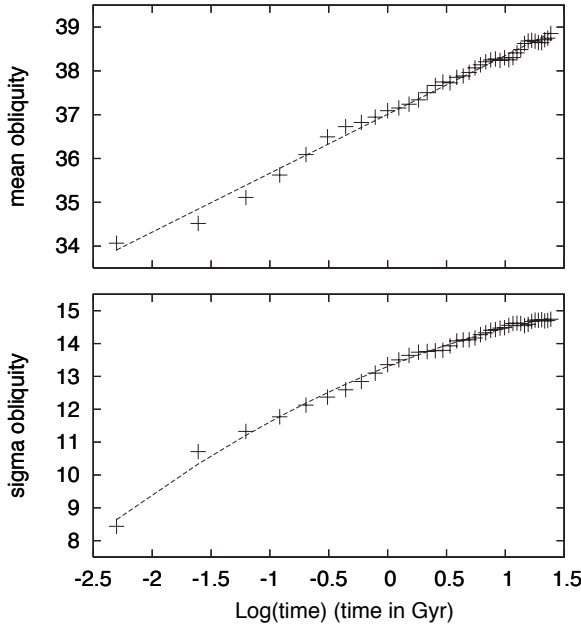
Figure 25: Evolution of the mean value \bar{\varepsilon} (top) and standard deviation \sigma_\varepsilon (bottom) for the obliquity of Mars. The statistics are made over 40 consecutive intervals of 100 Myr, for about 10000 orbits with close initial conditions. The mean obliquity is fitted with \bar{\varepsilon} = 37.007 + 1.345 \log(T) , while the standard deviation is fitted with \sigma_\varepsilon = 13.301 + 1.426 \log(T) - 0.259 \log^2(T) where T is in Gyr.
