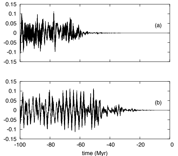
Figure 4: Stability of the solution for Mars' eccentricity. (a) Difference of the nominal solution La2003 with stepsize \tau = 5 \times 10^{-3} years, and La2003*, obtained with \tau^* = 4.8828125 \times 10^{-3} years. (b) Difference of the nominal solution with the solution obtained while setting J_2 = 0 for the Sun (instead of 2 \times 10^{-7} in the nominal solution).
