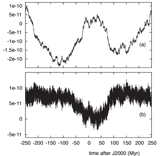
Figure 2: Integrals conservation. (a) relative variation of the total energy of the system versus time (in Myr) from -250 Myr to +250 Myr (with origin at J2000) after correction of the secular trend due to the tidal dissipation in the Earth-Moon system. (b) relative variation of the normal component of the total angular momentum.
