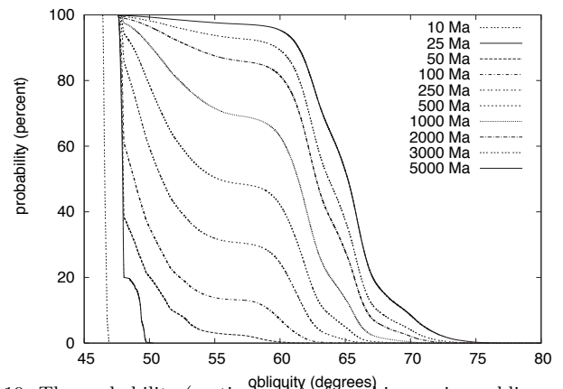
Figure 19: The probability (vertical axis) of reaching a given obliquity (horizontal axis) after a specified time if given by the different curves, for 10, 25, 100, 250, 500, 1000, 2000, 3000, 5000 Myr. The estimate is obtained with 200 different orbital solutions, with, for each of them, 1001 integrations for regularly spaced values of p ranging from p_0 - \delta p/2 to p_0 + \delta p/2 .
