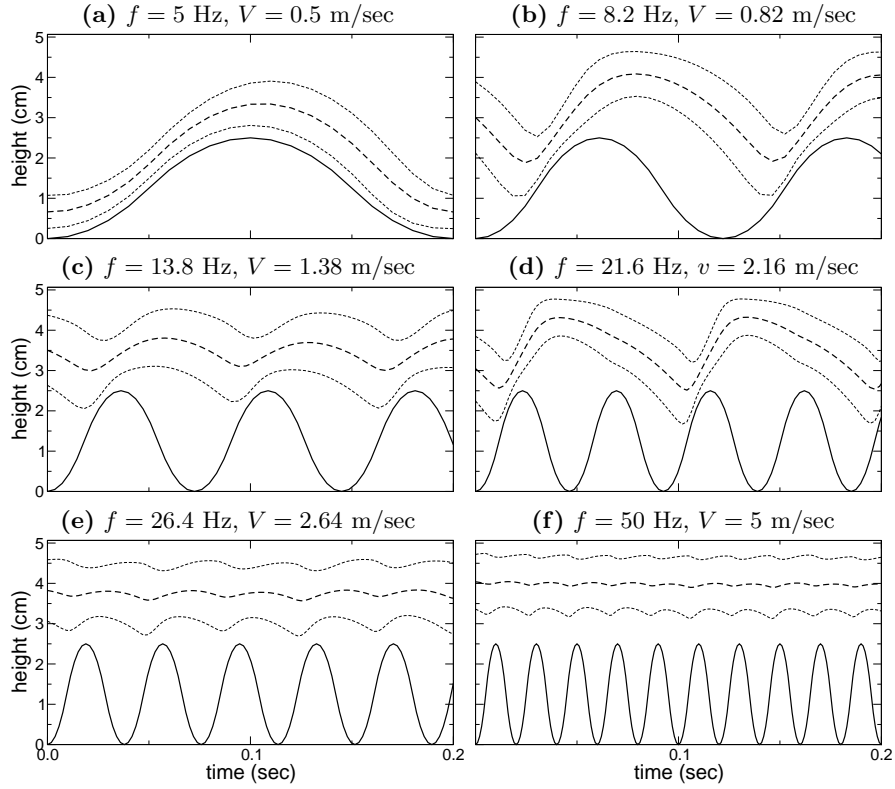
Fig. 12. The motion of the grains under gravity at various vibration frequencies during 0.2 seconds, for n = 6 , h - h_0 = 25 mm and r = r(v) . In all plots, the vertical axis is height, with the lower boundary at the piston's lowest point, and the upper boundary being the upper wall of the container. Solid line shows the position of the piston. The heavy dotted line shows the height y_{\text{cm}} of the center of mass. The upper and lower thin dotted lines show y_{\text{cm}} + \sigma_{\text{cm}} and y_{\text{cm}} - \sigma_{\text{cm}} respectively, where \sigma_{\text{cm}} is the standard deviation of the particle heights at a given instant. The majority of the particles are thus contained between the two thin dotted lines.
