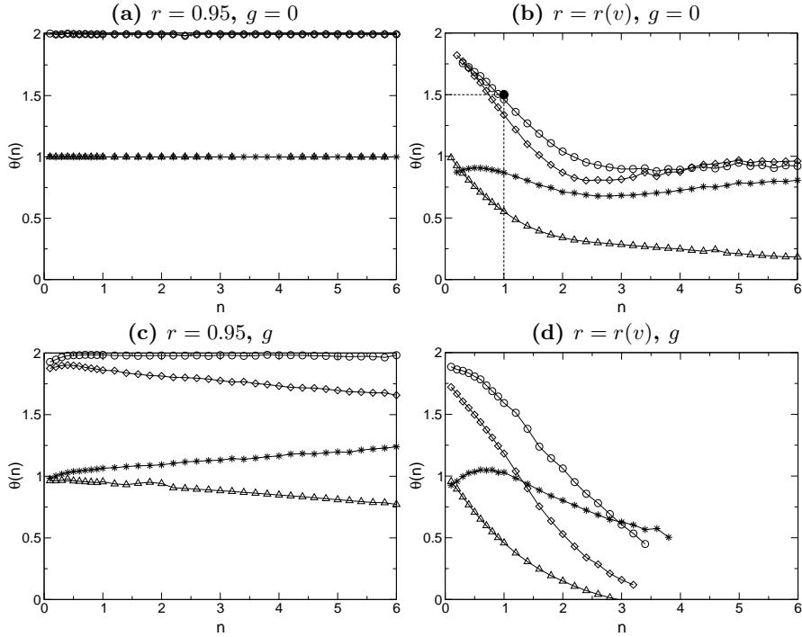
Fig. 4. The exponents \theta as a function of n which give the scaling of the granular temperature T ( \diamond ), collision frequency C_{\text{upper}} ( * ), mean impulses \Delta I ( \Delta ) and pressure P ( \circ ). All these quantities are proportional to V^{\theta(n)} . Without gravity: (a) for r = 0.95 and (b) for r = r(v) . With gravity: (c) for r = 0.95 and (d) for r = r(v) . The exponents are obtained by fixing n and performing eleven simulations, varying f from 10 Hz to 30 Hz. Then \log X (where X is the quantity being considered) is plotted against \log V . The resulting curve is always nearly a straight line (except for n > 3 in (d) – see text), and the exponent is calculated from a least squares fit. The pressure scaling point ( \bullet ) on (b) is from experiment [2] performed in low-gravity. See Fig. 3a (resp. Fig. 3b) for typical snapshots corresponding to n = 3 , g \neq 0 and r = r(v) (resp. r = 0.95 )
