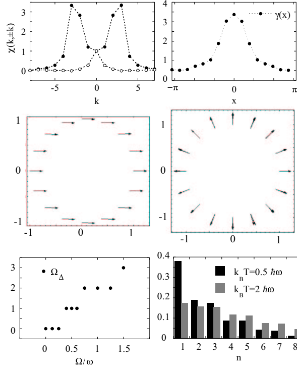
FIG.3. Stochastic Hartree-Fock calculations of the thermal equilibrium state of N_+ = N_- = 5 interacting fermions confined in a rotating ring of radius R at a temperature k_B T = 0.5 \hbar \omega with \omega = \hbar/mR^2 .
