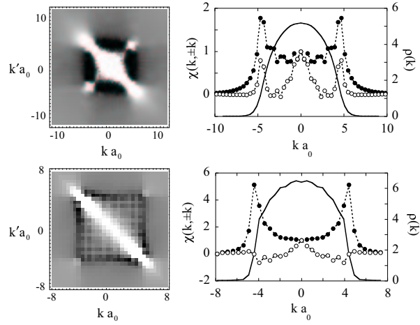
FIG.1. Cooper pairing correlations in a 1D system of N_+ = N_- = 10 interacting fermions in an harmonic trap at different temperatures k_B T = 2 \hbar \omega (top) and k_B T = 0.5 \hbar \omega (bottom). Left part: density plot of the momentum correlation function \chi(k, k') . Right part: momentum density profiles \rho(k) (solid line) and correlations \chi(k, \pm k) (dashed lines) relative to their value for k = 0 (open circles: \chi(k, k) , black disks: \chi(k, -k) ).
