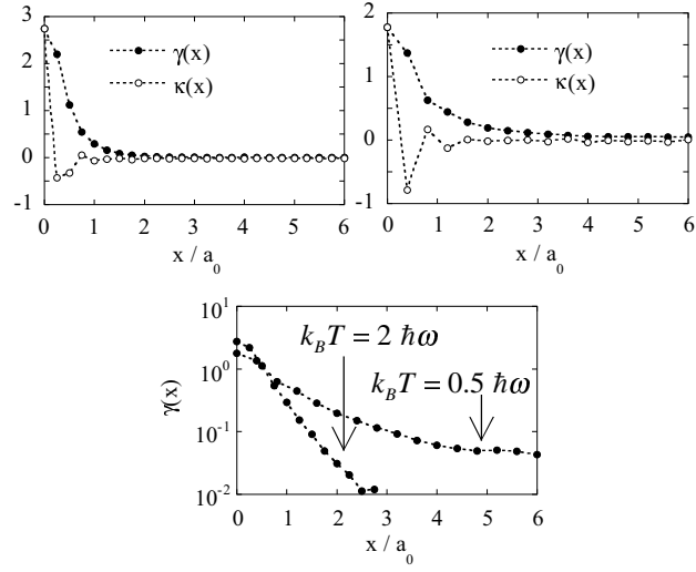
FIG.2. Upper part : exact non-local correlation functions \gamma(x) and \kappa(x) for N_+ = N_- = 10 harmonically trapped fermions at different temperatures k_B T = 2 \hbar \omega (left) and k_B T = 0.5 \hbar \omega (right). Lower part: comparison of the coherence function \gamma(x) for the two considered temperatures.
