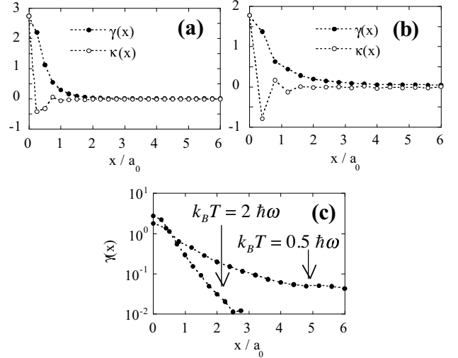
FIG. 2. Exact non-local correlation functions \gamma(x) and \kappa(x) for N_+ = N_- = 10 harmonically trapped fermions at different temperatures k_B T = 2 \hbar \omega (a) and k_B T = 0.5 \hbar \omega (b). (c): comparison of the coherence function \gamma(x) for the two considered temperatures.
