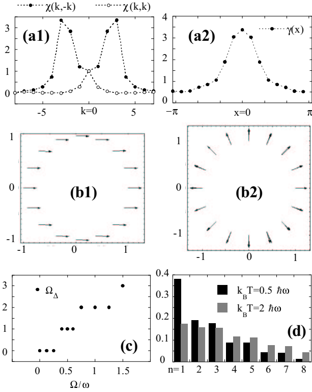
FIG. 3. Stochastic Hartree-Fock calculations of the thermal equilibrium state of N_+ = N_- = 5 interacting fermions confined in a rotating ring of radius R . In (a1,a2,b1,b2,c), the temperature is k_B T = 0.5 \hbar \omega with \omega = \hbar/mR^2 .
