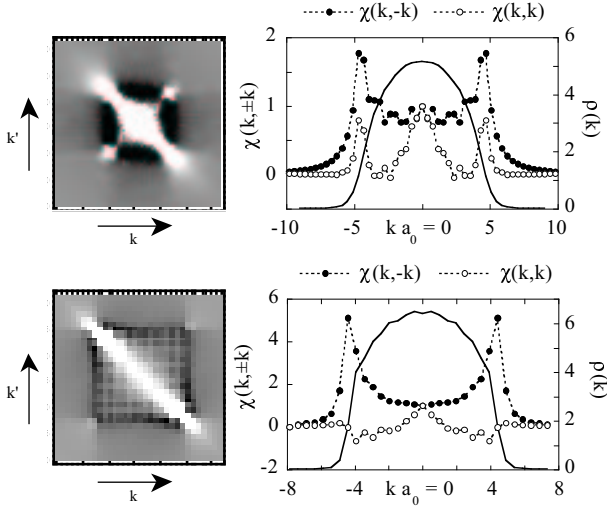
FIG. 1. Cooper pairing correlations in a 1D system of N_+ = N_- = 10 interacting fermions in an harmonic trap at different temperatures k_B T = 2 \hbar \omega (top) and k_B T = 0.5 \hbar \omega (bottom). Left part: density plot of the momentum correlation function. Right part: momentum density profiles \rho(k) (solid line) and correlations \chi(k, \pm k) (see text) relative to their value for k=0 .
