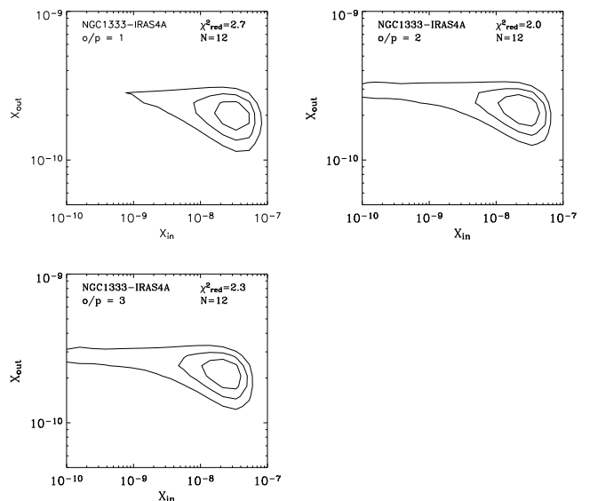
Fig. 10. \chi^2_{red} diagrams of NGC1333-IRAS4 for three different ortho to para ratios. The upper left, upper right and lower panels shows the \chi^2_{red} contours derived for an ortho to para ratio of 1, 2 and 3 respectively. Contours indicates the 1, 2 and 3\sigma confidence levels respectively.
