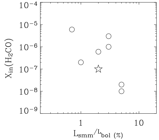
Fig. 13. Derived H 2 CO X_{\text{in}} abundances as a function of L_{\text{smm}}/L_{\text{bol}} . The star represent IRAS16293-2422.
