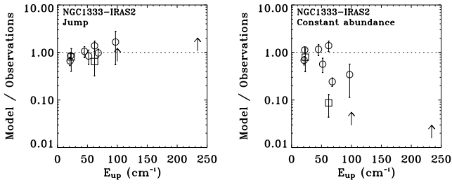
Fig. 8. Ratio of the model predictions over the observed fluxes of H 2 CO lines as a function of the upper energy of the line, for NGC1333-IRAS2. In the left panel a jump in the abundance (Tab. 6) is adopted, while in the right panel a constant abundance across the envelope is assumed. The circles and the squares represent H 2 12 CO and H 2 13 CO lines respectively. The arrows represent lower limits.
