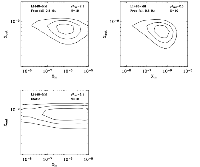
Fig. 9. \chi^2_{\text{red}} diagrams of L1448-MM for three different velocity profiles. The upper left and upper right panels show the \chi^2_{\text{red}} contours derived for a free falling envelope with a central mass of 0.3 and 0.8 M ⊙ respectively. The lower panel shows the static envelope case, with a 1 km s -1 turbulent velocity. Contours indicate the 1, 2 and 3 \sigma confidence levels respectively.
