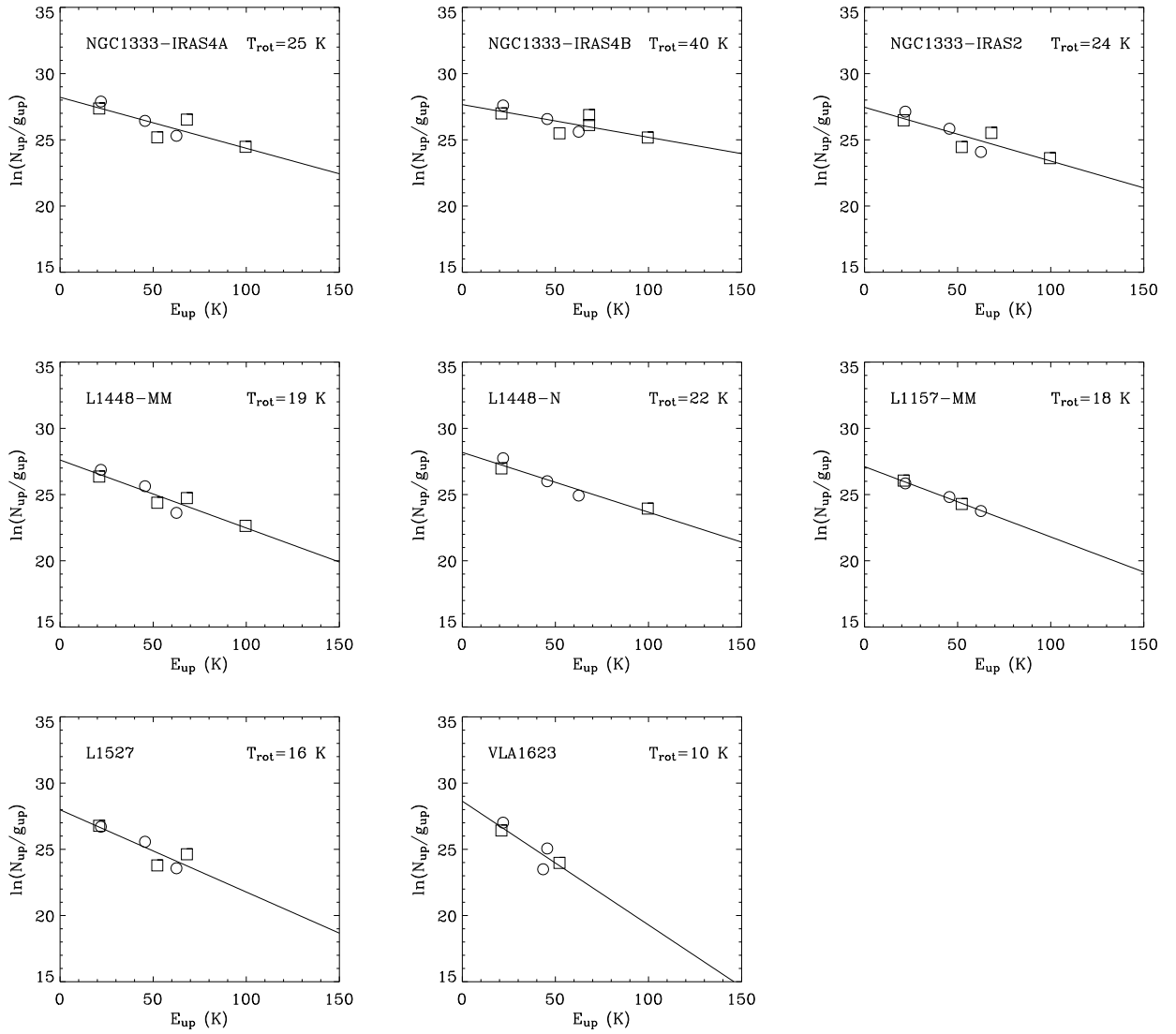
Fig. 4. H 2 CO rotational diagrams derived for the observed sources. Circles and squares mark the ortho and para H 2 CO transitions respectively. Fluxes of the para transitions have been multiplied by the ortho to para ratio, obtained by minimizing the \chi^2 between the observations and the predictions of the rotational diagram (see text). Solid lines show the best fit curves.
