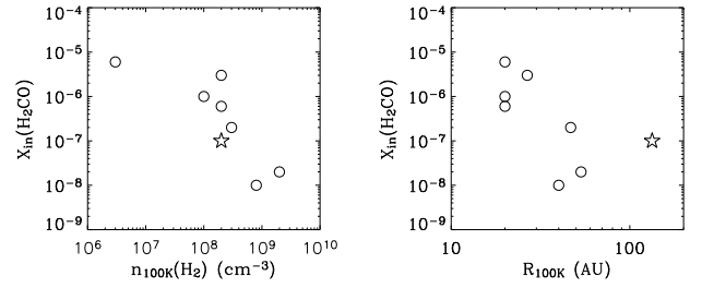
Fig. 12. Derived H 2 CO X_{\text{in}} abundances as a function of the density (left panel) and the radius (right panel) where T_{\text{dust}} = 100 K. The star represent IRAS16293-2422.
