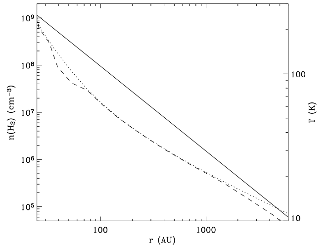
Fig. 6. Density (solid line), gas (dashed line) and dust (dotted line) temperature across the envelope of NGC1333-IRAS2.
