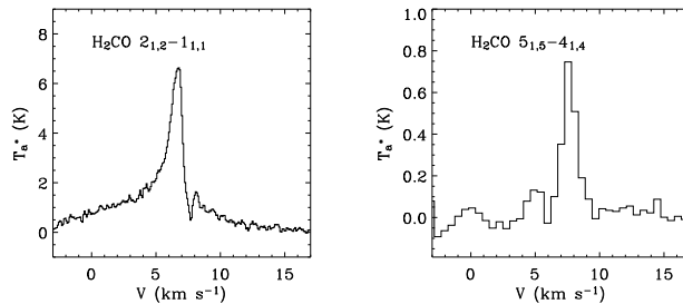
Figure 1: Typical exemple of formaldehyde lines observed towards NGC1333-IRAS4A
