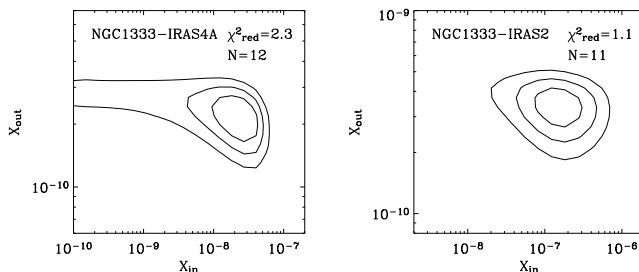
Figure 2: \chi^2 as a function of X_{\text{in}} and X_{\text{out}} for NGC1333-IRAS4A and NGC1333-IRAS2. The contour levels show the 1, 2 and 3 \sigma confidence level respectively.
