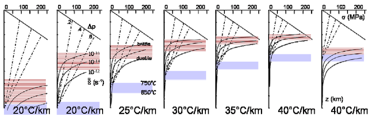
Fig. 2. Bulk rheology of the crust, using a power law rheology for amphibolites (Wilks & Carter, 1990) in case of geothermal gradient varying from 20 to 40 °C/km. Extensional brittle curve only is shown. Curves of viscous rheology under different strain rate ( 10^{-12} , 10^{-14} and 10^{-16} s ^{-1} ) are also indicated. It brackets the brittle/ductile transition (stippled in grey). Melting temperatures (in grey) are bracketed by the temperatures of muscovite (750 °C) and biotite (800°C) reactions. The buoyancy forces of a magma column originating at 800°C km in depth is represented using three values of density contrast (-0.2, -0.4 and -0.6 g/cm ^3 respectively). Experimental parameters of the ductile, power-law behaviour are the activation energy ( Q = 244 kJ/mole), the pre-exponential coefficient ( \log A = -9.11 (MPa/s) ^{1/n} ), the power coefficient ( n = 3.7 ). Temperature ( T ) is linked to the system by the perfect gas constant ( R = 8.31 J/mole/K). The geothermal gradients range from 20 to 40 °C/km.
