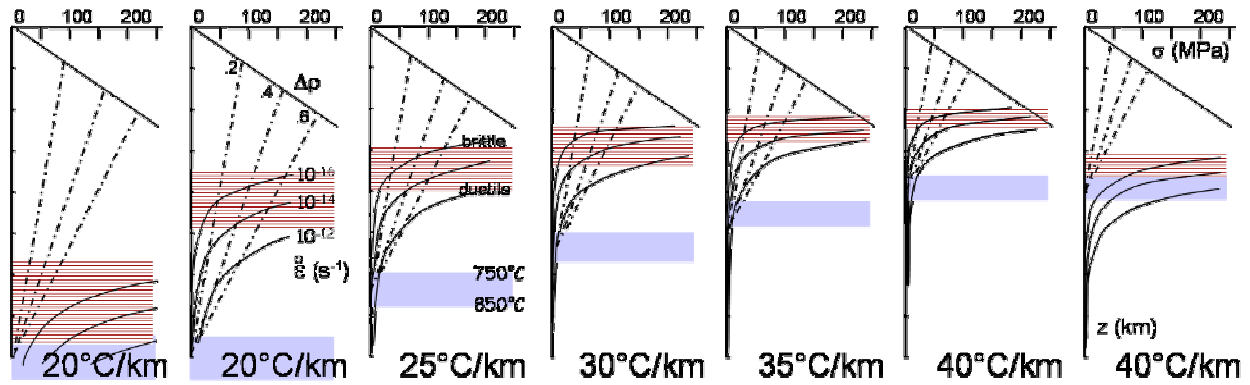
Fig. 2. Bulk rheology of the crust, using a power law rheology for amphibolites (Wilks & Carter, 1990) in case of geothermal gradient varying from 20 to 40 °C/km. Extensional brittle curve only is shown. Curves of viscous rheology under different strain rate ( 10^{-12} , 10^{-14} and 10^{-16} s ^{-1} ) are also indicated. It brackets the brittle/ductile transition (stippled in grey). Melting temperatures (in grey) are bracketed by the temperatures of muscovite (750 °C) and biotite (800°C) reactions. The buoyancy forces of a magma column originating at 800°C km in depth is represented using three values of density contrast (-0.2, -0.4 and -0.6 g/cm ^3 respectively). Experimental parameters of the ductile, power-law behaviour are the activation energy ( Q = 244 kJ/mole), the pre-exponential coefficient ( \log A = -9.11 (MPa/s) ^{1/n} ), the power coefficient ( n = 3.7 ). Temperature ( T ) is linked to the system by the perfect gas constant ( R = 8.31 J/mole/K). The geothermal gradients range from 20 to 40 °C/km.
