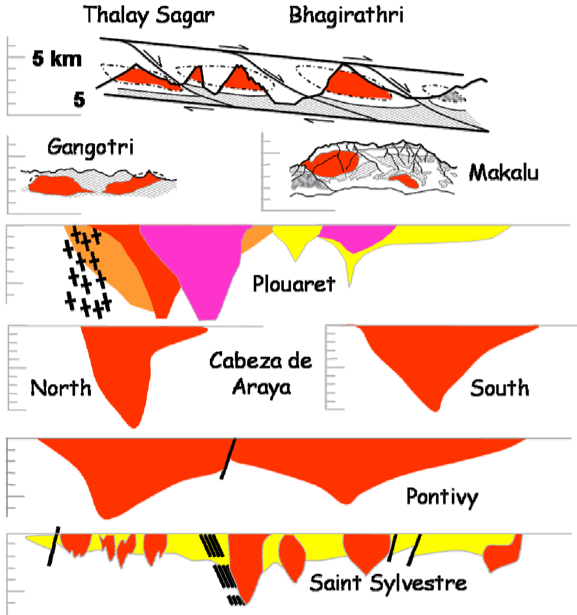
Fig. 4. Cross section through the High Himalayan granites redrawn from photos for the Bhagirathri and Thalay Sagar (Searle et al., 1993) Makalu (Lombardo et al., 1993) and Gangotri massif (Scaillet et al., 1995). In comparison, several cross sections, at the same scale, of Hercynian granites in Brittany (Plouaret, Pontivy), Massif Central (Saint Sylvestre) and Spain (Baseza de Araya) are provided from gravity data inversion (Améglio et al., 1997). A similar true scale (vertical = horizontal) is applied to all massifs
