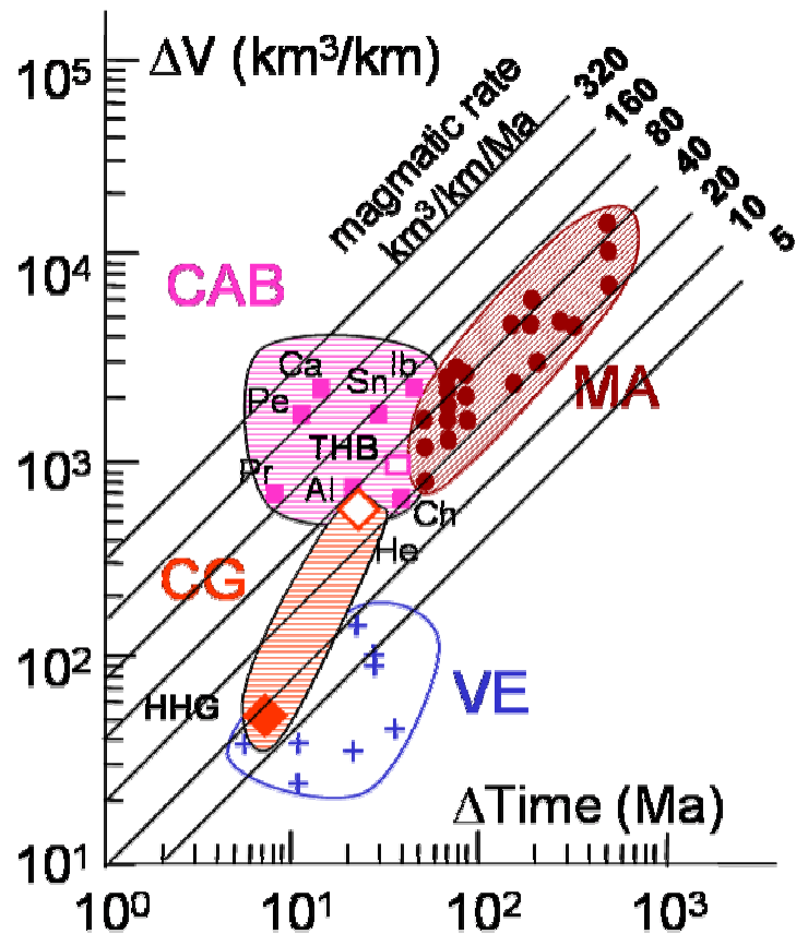
Fig. 1. Volume of magma and crust produced in magmatic arc. Crustal production in magmatic arcs (MA) from Marianas to Izu Bonin is redrawn from Reymer & Schubert (1984). Cretaceous calc-alkaline batholiths (CAB) from the eastern Pacific are indicated (Al: Alaska, Ca Canada, Ib Idaho-Boulder, Sn Sierra Nevada, Pr Peninsula Ranges, Pe Peru coastal batholith, Ch Chilean batholith). Volcanic eruptions (VE) are also indicated. Collision granites (CG) are shown for the Hercynian (He) and Himalayas (HHG). The Trans Himalayan Batholith (THB) plots within the field of the CAB.
