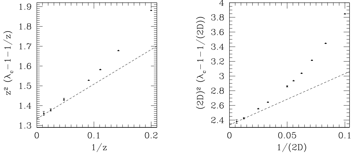
FIG. 4: Numerical data for the second-order correction in 1/z to \lambda_C(z) for the Cayley tree (left panel) and the hypercubic lattice (right panel). The critical value \lambda_C is obtained from numerical experiments on the conserved contact process (CPP), see main text. Data are plotted as z^2(\lambda_C(z) - 1 - 1/z) versus 1/z . The intercept a with the vertical axis ( z \rightarrow \infty ) compare very well with the theoretical predictions a = 4/3 — Eq. (56), left — and 7/3 — Eq. (55), right. Dashed lines are tentative linear fits (with fixed origin at 1/z = 0 ) of the data, whose slopes should be given by the O(1/z^3) expansion. The estimate of \lambda for each z was obtained through an extrapolation of data for finite numbers of particles N (up to 4000) to infinite N . For each value of N , we ran 10000 simulations and estimated error bars from the statistical fluctuations. The upper and lower values of \lambda_C(z; N = \infty) were then obtained through a linear fit of \lambda_C(z; 1/N) , and plotted at the extremities of the error bars.
