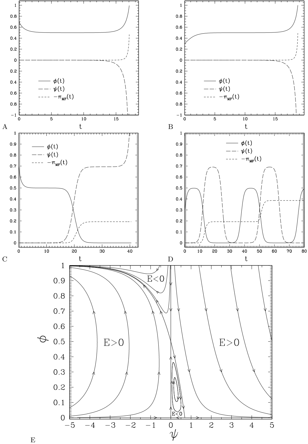
FIG. 3: Solutions of the mean-field equations of motion (34) for \lambda = 2 ( \rho^* = 1/2 ). A & B. For negative \psi(0) ( = -10^{-7} here), the solutions have a finite lifetime. After quickly reaching the most probable value of the density of particles, \rho^* , \phi(t) stays for a long time in the neighborhood of \rho^* but finally reaches unity, while \psi(t) \rightarrow -\infty . The action \pi_{MF} tends to a negative finite value; the main contribution to it comes from the final jump of \phi from \rho^* to 1. C. For positive \psi(0) ( = 10^{-8} here) and E > 0 , the lifetime is finite. After quickly reaching \rho^* , \phi(t) stays for a long time in its neighborhood but finally transits to the neighborhood of 0 where it stays again for a long time, while \psi(t) transits to \ln \lambda and stays close to it. Finally \psi(t) \rightarrow +\infty while \phi(t) \rightarrow 0 . \pi_{MF} tends to a negative finite value, the main contribution of which is accumulated during the transit. D. For positive \psi(0) > 0 ( = 10^{-8} here) and E < 0 , the solution is periodic. \phi(t) and \psi(t) oscillate between two values inside the [0, \rho^*] and [0, \ln(\lambda)] intervals, respectively, and the action diverges to -\infty by hops. E. Phase portrait with all types of solutions (oriented according to the time evolution). The phase space divides into four regions delimited by the solutions for which E = 0 (represented in bold lines); in each region the sign of E is indicated. The quasistationary state appears on this diagram as the crossing point ( \psi = 0, \phi = \rho^* ) of two solutions with E = 0 : it is stable along the \phi direction but instable along the \psi direction.
