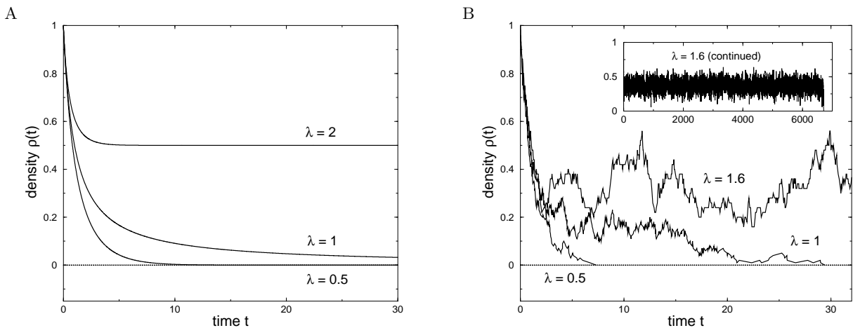
FIG. 1: Profiles of the density \rho of particles versus time t for the Contact Process over a complete graph of N vertices, initially filled with particles ( \rho(0) = 1 ). A. Thermodynamic limit, N \rightarrow \infty . From bottom to top: subcritical ( \lambda < \lambda_C = 1 , the density exponentially relaxes toward zero), critical ( \lambda = \lambda_C , the density algebraically decays to zero as \rho(t) \sim t^{-1} ), and supercritical ( \lambda > \lambda_C , the density exponentially relaxes to a finite value, \rho^* = 1 - 1/\lambda ) cases. The density obeys a deterministic evolution equation (36), and no fluctuation is present. B. Finite size lattice, with N = 100 sites. CP is a stochastic process, and the density profiles vary from run to run (we show here one run for each value of \lambda ). The density quickly relaxes to zero (subcritical regime) or a finite value (supercritical regime). In the latter case, the system is trapped in a metastable regime where the density fluctuates for a very long time around its plateau value (Inset, notice the difference of time scale), till a large fluctuation drives the density to the zero value.
