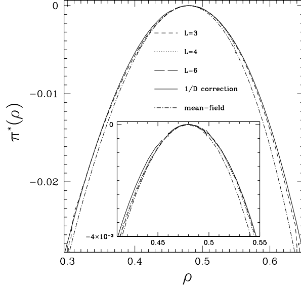
FIG. 5: Comparison, for D = 6 and \lambda = 2 , between the 1/D predictions for the large deviation function \pi^*(\rho) and numerical results for CP on hypercubic lattices with periodic boundary conditions of linear sizes L = 3, 4 and 6 . All curves were horizontally and vertically translated so that their maxima have the same coordinates \rho^*, \pi^* = 0 . Due to the relatively high dimensionality of these systems, the range of values of \rho explored during the simulations is very concentrated around \rho^* unless L is small. Note that the curves for different lattice sizes, once translated, seem to depend only weakly on L . Inset: blow-up of the top region; data compare well with the 1/D theoretical result (continuous line), and are clearly distinct from the mean-field result (dashed-dotted line).
