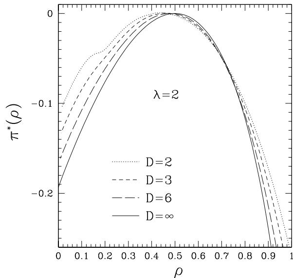
FIG. 2: The large deviation function \pi^* for the density of particles in CP with parameter \lambda = 2 for the D -dimensional hypercubic lattice. The D \rightarrow \infty curve corresponds to the mean-field limit, and coincides with the case of the complete graph over N \rightarrow \infty sites. Plot of the predicted value of \pi^*(\rho) at the order 1/D for D = 6, 3 and 2 are obtained with the expansion of Section IV. The nonconvexity of the curve for D = 2 shows the inaccuracy of the truncation to first order of our 1/D expansion in this range of densities.
