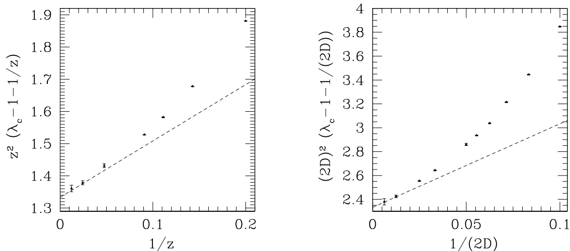
FIG. 4: Numerical data for the second-order correction in 1/z to \lambda_C(z) for the Cayley tree (left panel) and the hypercubic lattice (right panel). The critical value \lambda_C is obtained from numerical experiments on the conserved contact process (CPP), see main text. Data are plotted as z^2(\lambda_C(z) - 1 - 1/z) versus 1/z . The intercept a with the vertical axis ( z \rightarrow \infty ) compare very well with the theoretical predictions a = 4/3 — Eq. (56), left — and 7/3 — Eq. (55), right. Dashed lines are tentative linear fits (with fixed origin at 1/z = 0 ) of the data, whose slopes should be given by the O(1/z^3) expansion. The estimate of \lambda for each z was obtained through an extrapolation of data for finite numbers of particles N (up to 4000) to infinite N . For each value of N , we ran 10000 simulations and estimated error bars from the statistical fluctuations. The upper and lower values of \lambda_C(z; N = \infty) were then obtained through a linear fit of \lambda_C(z; 1/N) , and plotted at the extremities of the error bars.
