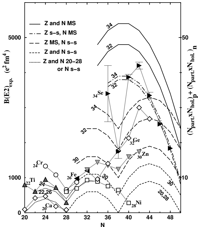
FIG. 5: Joined by dotted grey lines and using different symbols, experimental B(E2)_{\text{exp}} values for Ca, Ti, Cr, Fe, Ni, Zn, Ge and Se isotopes from [10]. For sake of legibility only a half of the error bars of the Se isotopes (when larger than the symbols) is reported. For the error bars on the other nuclei see fig.1. Several of the calculated B(E2)_{\text{approx}} curves presented in fig.3 are reported. For all the curves the proton number is explicitly given.
