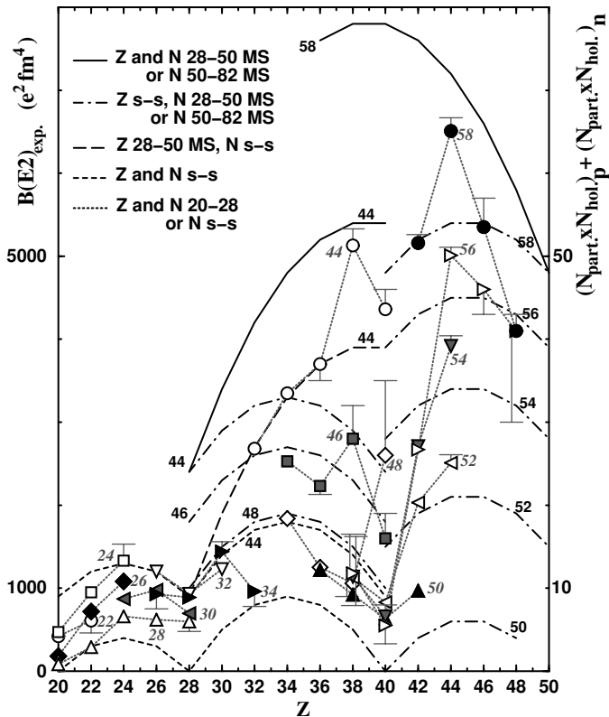
FIG. 7: Joined by dotted grey lines and using different symbols experimental B(E2)\uparrow values along the isotonic series with neutron number from 22 up to 36, and from 44 up to 58. All the experimental values are from [10]. For sake of legibility only a half of the error bars, when larger than the symbols, are reported. In different black lines are reported several calculated curves. For all the curves the neutron number is explicitly indicated.
