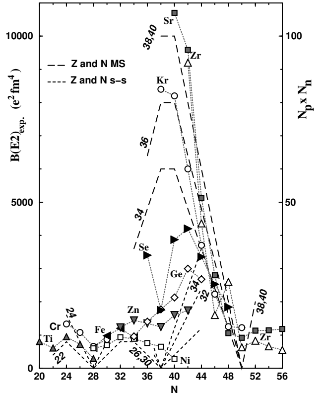
FIG. 11: Joined by dotted grey lines experimental B(E2)\uparrow values of Ti (full grey triangles), Cr (empty circles), Fe (full black left triangles), Ni (empty squares), Zn (full grey triangles right), Ge (empty diamonds), Se (full black triangles right), Kr (empty circles), Sr (full grey squares) and Zr (empty triangles up) isotopes. For the error bars see fig.4,5. The calculated product of number of protons and neutrons (or holes for both types of particles past the mid-shells) N_p \times N_n are reported : in long-dashed line for the double major shell, protons and neutrons, in short-dashed line for both sub-shell closures ( N=38 and Z=40 ) which is, for Z \leq 34 , the same as with the sub-shell closure N=38 and full major shell in protons. For all the curves the proton number is explicitly indicated.
