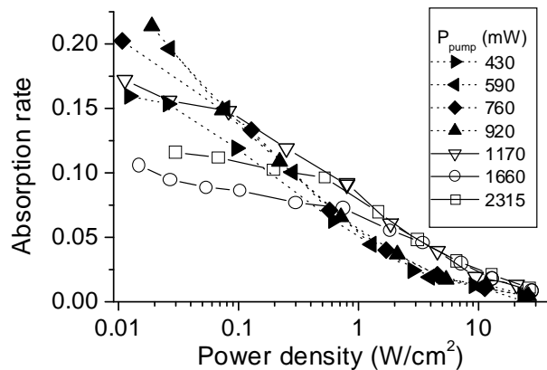
Fig. 10 Absorption rates versus power densities for the loop mirror oscillator (same data sets as in Fig. 9, but without normalization to maximum values).
