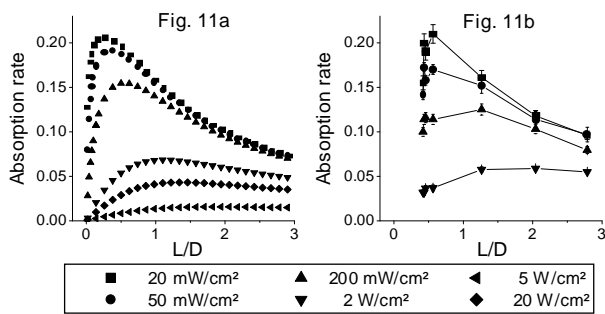
Fig. 11 Absorption versus laser FWHM L (scaled to the Doppler width D ), for various light power densities. Fig. 11a: Computed results using the phenomenological OP model [10]. Fig. 11b: Experimental measurements with the loop mirror oscillator (data sets extracted from Fig. 10).
