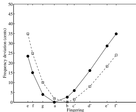
Fig. 20. Frequency deviation associated with the register hole in the case of a real clarinet (i.e restricting our optimization to fingering from e to f': above f', fingerings are modified to ensure the well tuning and the third resonance is used). Optimal positions are \ell_{\star}^{(1)} = 133.7 \text{ mm} (□) and \ell_{\star}^{(2)} = 145.0 \text{ mm} (●)
