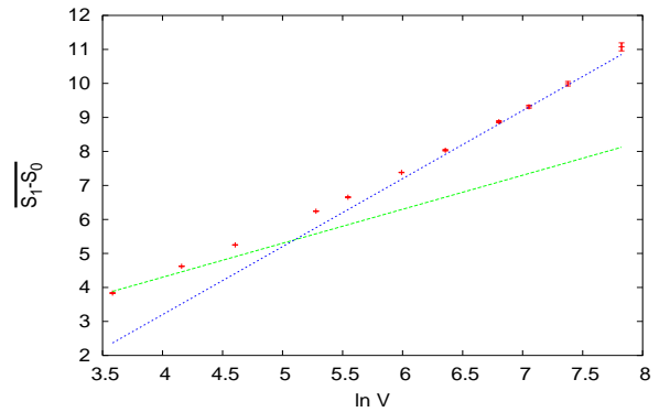
FIG. 3: \overline{S(E_0 + 4J) - S(E_0)} versus \ln(V) and the functions \ln(V) and 2\ln(V) .
