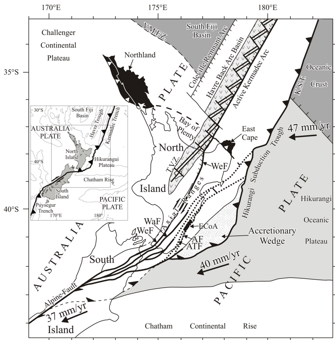
Figure: Geodynamic pattern of North Island, New Zealand. White areas are of continental and arc lithosphere. Light grey area corresponds to thickened oceanic lithosphere. Light grey area with V pattern is the active volcanic zone of the back-arc domain. Dark grey areas are underlain by oceanic lithosphere. Black areas image material obducted along the north coast (Northland and East Cape), then dragged along the East Coast (East Coast Allochthon: ECoA). Heavy solid lines are major active faults (WeF: Wellington Fault, WaF: Wairarapa Fault). Heavy dotted lines are faults with decreasing or no activity. V.M.F.Z.: Vening Meinesz Fracture Zone, T.V.Z.: Taupo Volcanic Zone, K.S.T.: Kermadec Subduction Trench.
