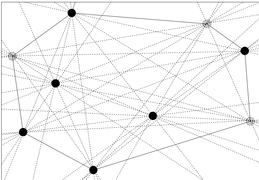
Figure 1: An orchard having 3 cherry- and 6 plumbtrees in generic positions
