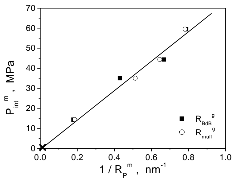
FIG. 4 – Mean intrusion pressure of water as a function of the inverse pore radius determined by nitrogen sorption for the four grafted materials. (The line is a guide for the eyes, the cross represents the origin).
