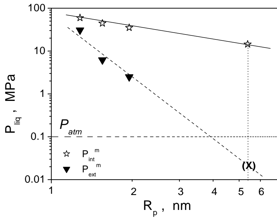
FIG. 5 – Mean intrusion and extrusion pressure of water as a function of the mean pore radius R_{muff}^g .
