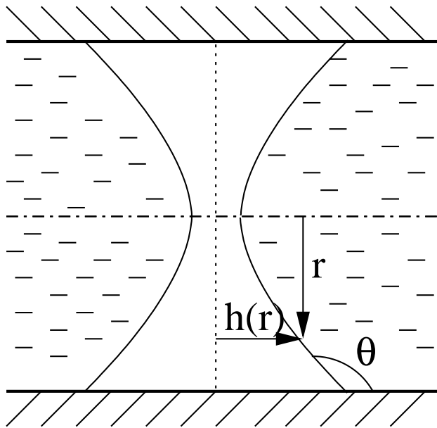
FIG. 7 – Definition of the function h(r) describing a nucleus with cylindrical symmetry.
