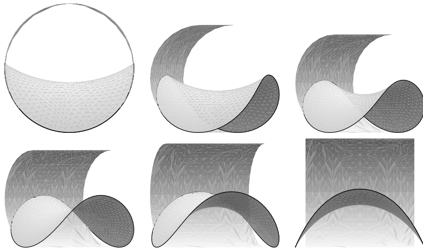
FIG. 10 – Several views of a vapor bubble in contact with the pore wall for an equilibrium contact angle fixed to 120^\circ . Each picture is obtained from the previous one by an 18^\circ rotation to the left. Only one half of the cylinder has been displayed. The solid-vapor interface is not represented.
