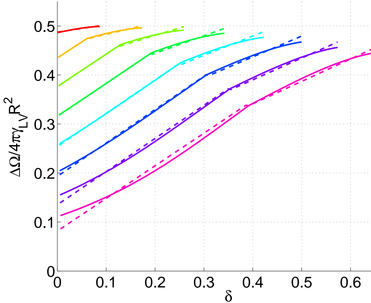
FIG. 13 – Reduced energy barrier as a function of \delta obtained in the most favourable configuration (bubble or cylindrical bump). From left to right, the values of the contact angle \theta are 95^\circ , 100^\circ , 105^\circ , 110^\circ , 115^\circ , 120^\circ , 125^\circ , 130^\circ . The dashed lines are the best fit of each curve with a piecewise linear function, as described in the text.
