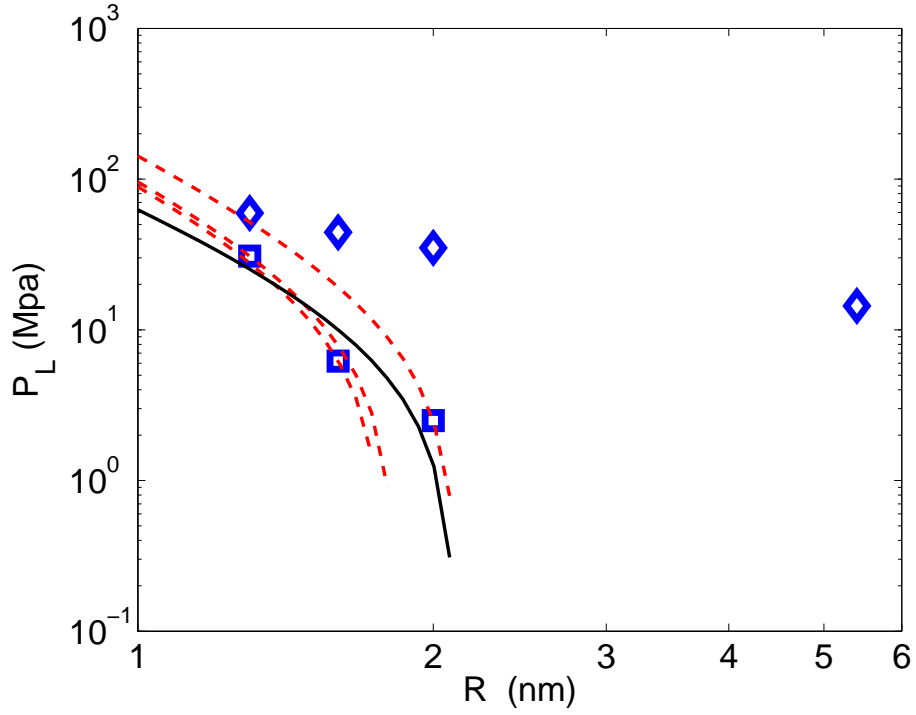
FIG. 14 – Extrusion (squares) and intrusion (diamonds) pressure versus pore radius. Dotted lines : theoretical curves for the extrusion obtained using equation 18, and assuming values of \Delta\Omega = 135k_B T , \Delta\Omega = 142k_B T and \Delta\Omega = 190k_B T for the extrusion process. Full line : theoretical curve obtained using equation 20, with \Delta\Omega = 35k_B T and \lambda = -2.4 \times 10^{-11} \text{ J.m}^{-1} .
