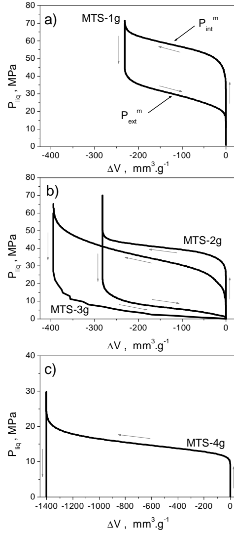
FIG. 3 – Intrusion/extrusion of water for the four grafted materials at 298 K : the pressure of the liquid P_{liq} is reported as a function of the volume variation \Delta V expressed per gram of bare silica.
