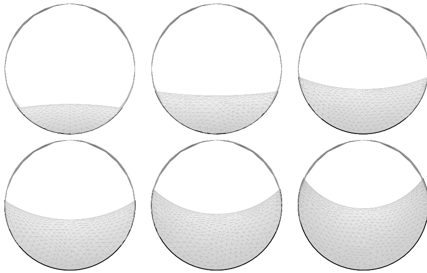
FIG. 9 – Views of the vapour bubble growing on the surface of a cylindrical pore, for various values of the volume. Camera viewing axes is the cylinder axes. The contact angle is 120^\circ . Only the liquid-vapour interface is displayed.
