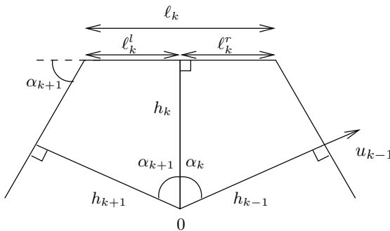
FIGURE 1. Notations for a convex polygon.
