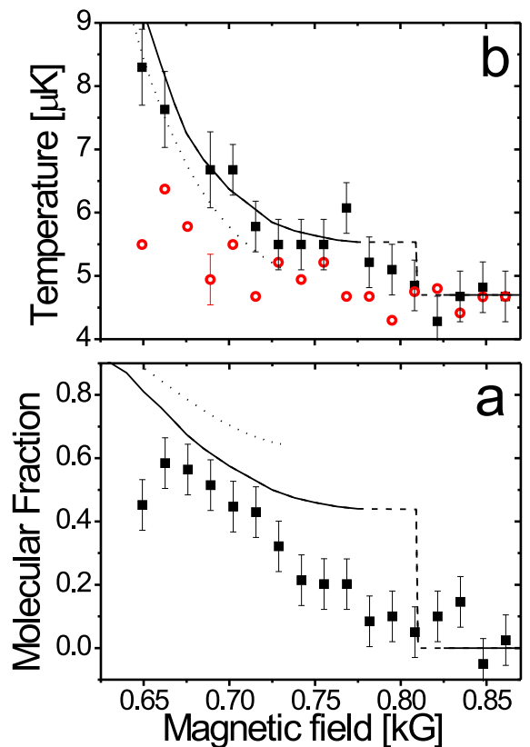
FIG. 2: a: fraction of atoms in molecular bound state, (N_3 - N_2)/N_3 , versus magnetic field at position 2 in Fig. 1. b: Corresponding atom temperature at position 2 (squares) and 3 (circles). Solid (dotted) line corresponds to the non-interacting (interacting) thermodynamical model described in text.
