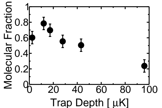
FIG. 3: Fraction of atoms bound in a molecule as a function of the depth of the dipole trap for B = 689 G, a = 78 nm, E_b = 12 \mu\text{K} .
