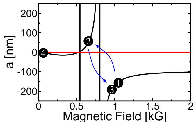
FIG. 1: Calculated scattering length a versus magnetic field for the 6 Li |F, m_F\rangle = |1/2, 1/2\rangle, |1/2, -1/2\rangle mixture near the 810 Gauss Feshbach resonance. Scanning over the resonance from 1 to 2 in 50 ms produces cold and trapped molecules with an efficiency up to 85%, resulting in an almost complete disappearance of the atomic signal at 2. Reversing then the scan to the initial position re-establishes the initial atomic signal. In all cases, atoms are detected and imaged at position 4 after abrupt switch-off of the B field.
