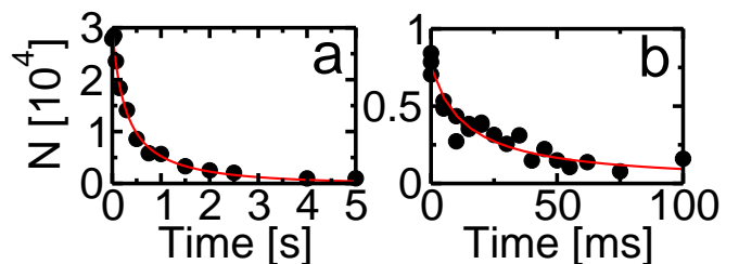
FIG. 4: Decay of \text{Li}_2 molecules in the optical trap for two values of the magnetic field: (a) B = 689 G, a = 78 nm, (b) B = 636 G, a = 35 nm. Note the difference in time scales. Solid lines are fits with 2-body and 1-body processes giving initial time constants of 500 ms in (a) and 20 ms in (b).
