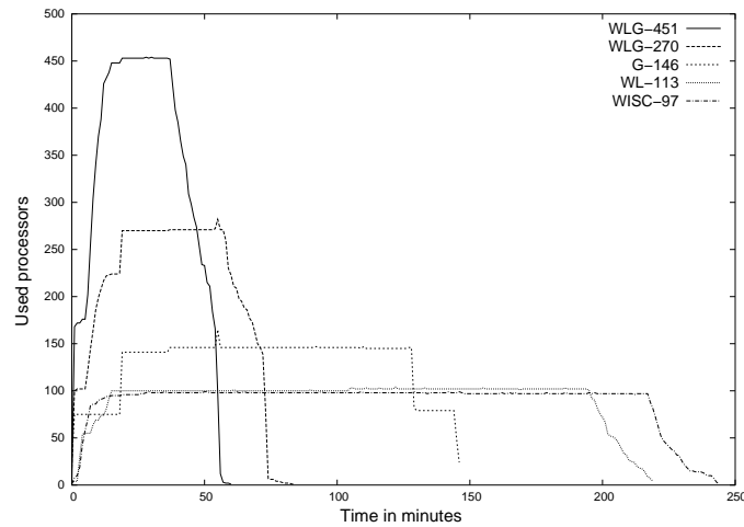
FIG. 3: Processors utilization.
