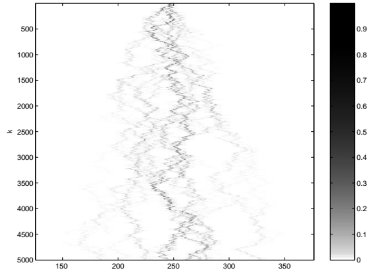
Figure 1: a sample of the measure-valued process \{\nu_k^{(20)}, 0 \leq k \leq 5000\}
