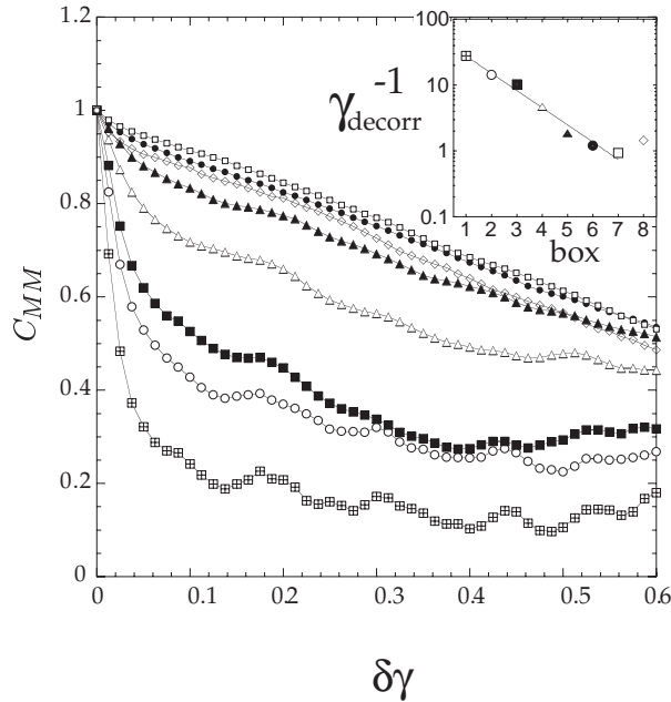
FIGURE 12. Run 2 (stationary flow): autocorrelation C_{M_{r\theta}M_{r\theta}} of the cross-component M_{r\theta} . Box 1: crossed boxes , box 2: open circles , box 3: closed squares , box 4: open triangles , box 5: closed triangles , box 6: closed circles , box 7: open squares , box 8: diamonds . Insert: initial decorrelation rate \gamma_{\text{decorr}}^{-1} for each box (eq. 4.6).
