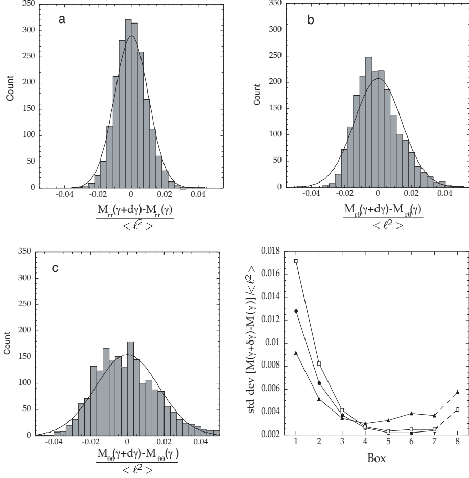
FIGURE 10. Run 2 (stationary flow): statistics for the increments of the texture tensor \overline{M} . (a) Histogram of increments of M_{rr} in box 1, again expressed in units of \langle \ell^2 \rangle . Solid line is a Gaussian with the same standard deviation and zero average. (b, c) The same for M_{r\theta} and M_{\theta\theta} . (d) Standard deviation of increments of \overline{M} versus box number (closed triangles: M_{rr} ; open squares: M_{\theta\theta} ; closed circles: M_{r\theta} ). Since the fluctuations in box 8 are extremely small (see Fig. 3), the data are noisy: image filtering and thresholding would have been required to obtain a statistically significant value.
