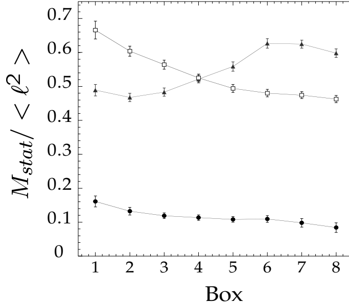
FIGURE 6. Run 2 (stationary flow): texture tensor \overline{\overline{M}}_{stat} versus box number. The components of \overline{\overline{M}} (closed triangles: M_{rr} ; open squares: M_{\theta\theta} ; closed circles: M_{r\theta} ), again expressed in units of \langle \ell^2 \rangle , are averaged over the four quarters of the whole foam, and also over time (2000 pictures).
