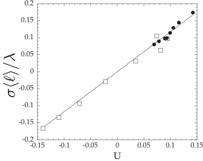
FIGURE 9. Run 2 (stationary flow): Hooke relation. The deviatoric part of the capillary stress \overline{\sigma}^{cap} , expressed in units of \lambda/\langle\ell\rangle , plotted versus the corresponding components of \overline{U} (closed circles: \sigma_{r\theta}^{cap} versus U_{r\theta} ; open squares: \sigma_{rr}^{cap} - \sigma_{\theta\theta}^{cap} versus U_{rr} - U_{\theta\theta} ). Each data point comes from Figs. (7) and (8), i.e. it derives from averages at one position in the foam. The solid line is a linear fit through all points, slope 2\mu\langle\ell\rangle/\lambda = 1.17 \pm 0.04 .
