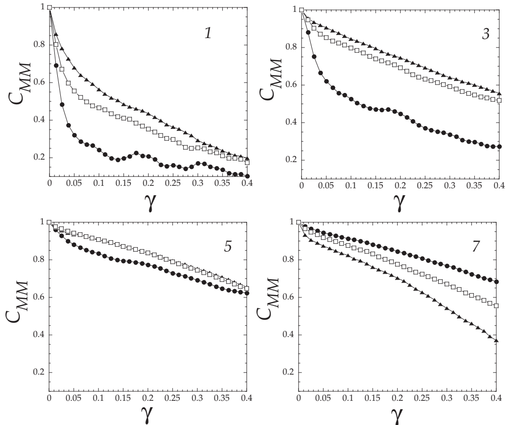
FIGURE 11. Run 2 (stationary flow): temporal autocorrelation C_{MM} of texture tensor \overline{\overline{M}} (eq. 4.5), versus \delta\gamma , in boxes 1, 3, 5, 7 (closed triangles: M_{rr} ; open squares: M_{\theta\theta} ; closed circles: M_{r\theta} ). We recall that the total applied shear \gamma is proportional to time, not to the local shear in each box (eq. 2.1).
