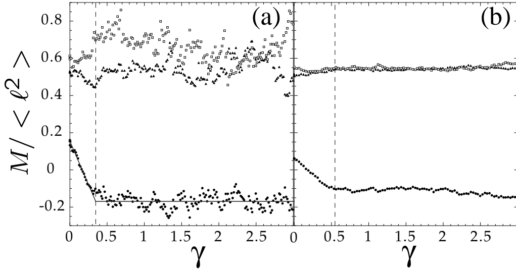
FIGURE 3. Run 1 (transient regime): texture tensor \overline{\overline{M}} versus the applied shear strain \gamma . The components of \overline{\overline{M}} defined in eq. (3.12) and measured from the first 200 images ( closed triangles : M_{rr} ; open squares : M_{\theta\theta} ; closed circles : M_{r\theta} ) are expressed in units of the average length of the bubble wall, \langle \ell^2 \rangle . (a) Innermost box (number 1): each point represents one image; (b) outermost box (number 8): for clarity, we show only every second image. The vertical dashed line marks the cross-over \gamma_Y between the transient and stationary regimes, defined by the intersection between the straight line and the zero slope line fitting M_{r\theta} in the transient and stationary regimes, respectively (solid lines in (a)).
