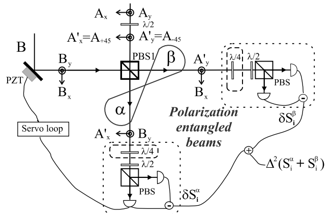
FIG. 3: Set-up for non separable beams generation. Inserting the quarter-wave plates (or not) allows for measuring the fluctuations of S_3^\alpha + S_3^\beta (or S_2^\alpha + S_2^\beta ). The servo loop is used to lock the B field phase to the squeezed quadrature angle.
