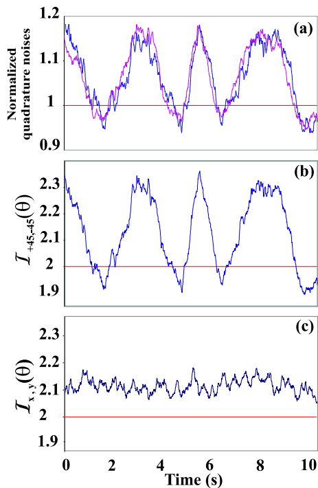
FIG. 2: (a) Quadrature noise spectra of A_x and iA_y , at a frequency of 5 MHz, when the relative phase \theta between the LO and the mean field mode is varied in time. (b) Direct measurement of \mathcal{I}_{+45,-45}(\theta) . (c) Corresponding measurement of \mathcal{I}_{x,y}(\theta) .
