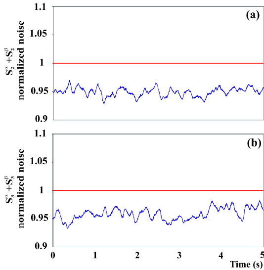
FIG. 4: Normalized noises at 5 MHz of S_2^\alpha + S_2^\beta (a) and S_3^\alpha + S_3^\beta (b), the phase \theta_B being locked with the value of the squeezed quadrature angle \theta_{sq} .
