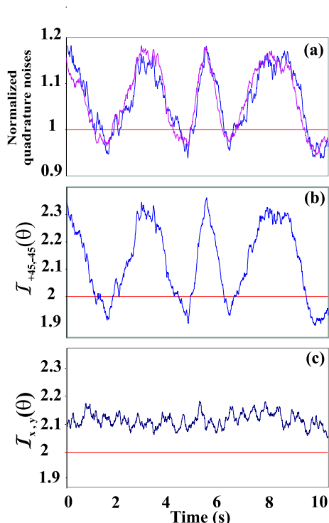
FIG. 3: (a) Quadrature noise spectra of A_x and iA_y , at a frequency of 5 MHz, when the relative phase \theta between the LO and the mean field mode is varied in time. (b) Direct measurement of \mathcal{I}_{+45,-45}(\theta) . (c) Corresponding measurement of \mathcal{I}_{x,y}(\theta) .
