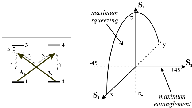
FIG. 1: Left : X-like atomic level structure. Right : Poincaré sphere for the Stokes parameters. While the sum of squeezing is maximal in the (S_1, S_3) plane, entanglement is optimal along the S_2 -axis.
