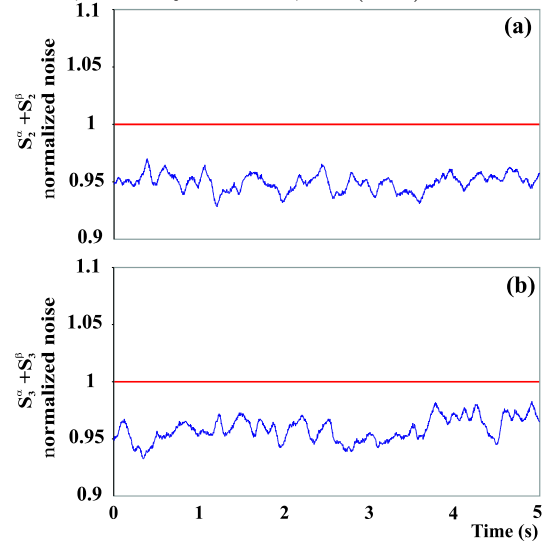
FIG. 5: Normalized noises at 5 MHz of S_2^\alpha + S_2^\beta (a) and S_3^\alpha + S_3^\beta (b), the phase \theta_B being locked with the value of the squeezed quadrature angle.
