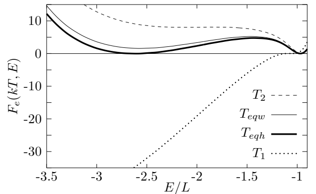
FIG. 7: Graphs of F_e(kT, E) = -\log N_{rw}(kT, E) for q = 5, \sigma = 0.3, N = 400 , at four characteristic temperatures: T_1, T_2, T_{eqh} and T_{eqw} = T_c denote the temperatures of the two metastable states, the temperature of equal peaks heights, and that of equal peaks weights, respectively. E/L denotes the energy per spin.
