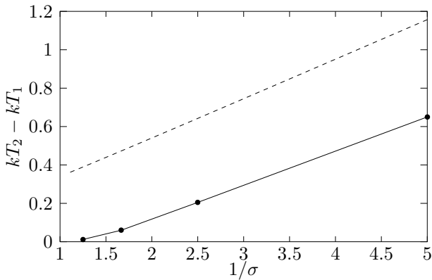
FIG. 11: Difference between temperatures of metastability dkT_m = kT_2 - kT_1 vs. 1/\sigma for q = 7 (disks connected by solid lines). Errors are smaller than the size of dots. MF prediction is shown for comparison (dashed line).
