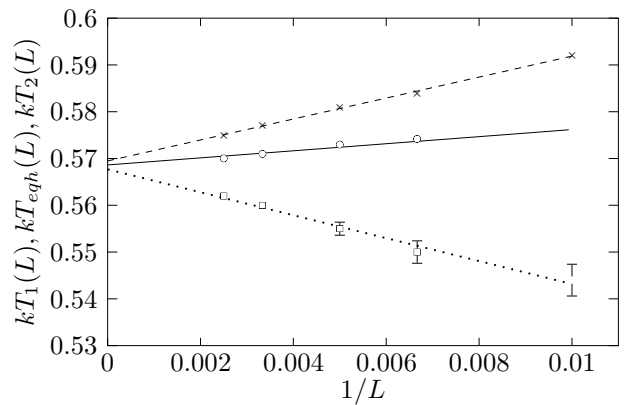
FIG. 14: Linear fit of finite size temperatures vs. 1/L for q = 9, \sigma = 1.0 . Dotted, solid, and dashed lines correspond to kT_1 , kT_{eqh} and kT_2 respectively. Error bars are smaller than the size of dots, except where explicitly indicated. In the limit L \rightarrow \infty , the difference between temperatures of metastability tends to 0.0012. Within our error bars, the transition is thus clearly not of the first-order.
