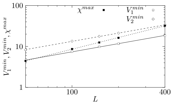
FIG. 15: Fit of V_1^{min} , V_2^{min} and \chi^{max} vs. L on a log-log scale, for L = 50, 100, 150, 200, 400 ( q = 5, \sigma = 0.9 ). Errors are smaller than the size of dots.
