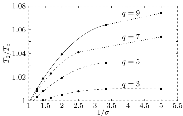
FIG. 12: T_2/T_c vs. 1/\sigma for q = 3, 5, 7, 9 . Solid lines indicate polynomial fits. Dotted lines are guides to the eyes. Error bars are smaller than the size of dots, except where explicitly indicated.
