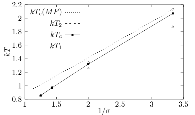
FIG. 9: Spinodal curve for 0.3 \leq \sigma \leq 0.8 ( q = 5 ). The transition temperature T_c is indicated by filled squares, and limits of metastability T_1 and T_2 by triangles and diamonds, respectively. Errors are smaller than the size of dots, and lines are drawn to guide the eyes. The dotted line shows the transition temperature as predicted by MF theory.
