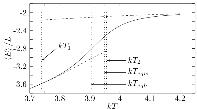
FIG. 8: Average energy per spin for q = 3, \sigma = 0.2, L = 400 , computed over both phases (solid line), ordered phase only (lower dashed line) and disordered phase only (upper dashed line). Vertical dotted lines indicate the four characteristic temperatures: from left to right, lower limit of metastability ( kT_1 ), transition temperatures (equal heights kT_{eqh} , then equal weights kT_{eqw} ), upper limit of metastability ( kT_2 ).
