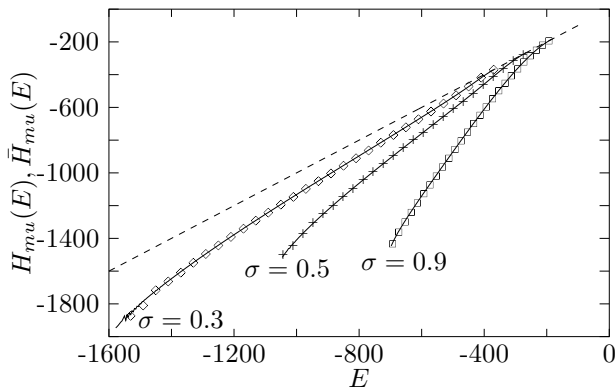
FIG. 3: Dots indicate the initial guesses \bar{H}_{mu}(E) that were fed into the iteration scheme at L = 400 , q = 5 , and \sigma = 0.3(\diamond), 0.5(+), 0.9(\square) . Each initial guess was computed using Eq. (5), i.e. by scaling a true estimate obtained at L = 200 . Solid lines show true estimates H_{mu}(E) as obtained after the whole iteration scheme at L = 400 converged. The straight dashed line sketches the original Hamiltonian, i.e. H_{mu}(E) = E .
