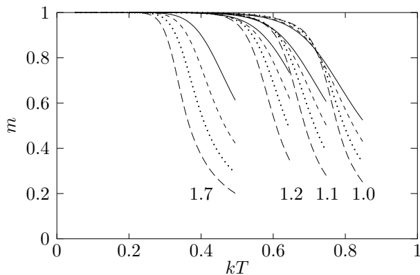
FIG. 18: Magnetization vs. kT for \sigma = 1.0, 1.1, 1.2 and 1.7 from right to left. Solid, dashed, dotted and long-dashed styles refer to L = 50, 100, 200 and 400 respectively.
