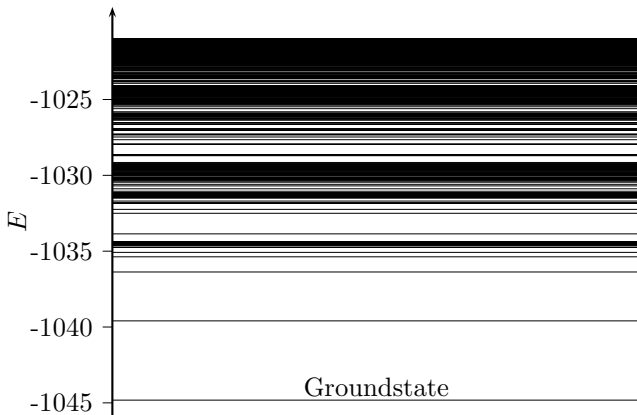
FIG. 2: Lowest energy levels for q = 5, \sigma = 0.5, N = 400 , computed by sorting energy samples from a long simulation run. Each level is drawn as an horizontal line.
