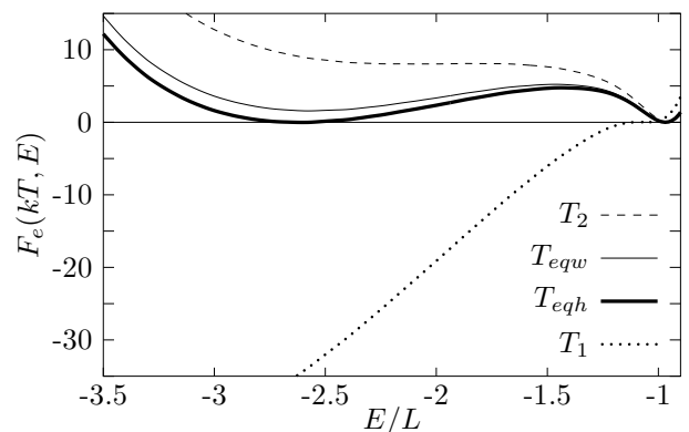
FIG. 7: Graphs of F_e(kT, E) = -\log N_{rw}(kT, E) for q = 5, \sigma = 0.3, N = 400 , at four characteristic temperatures: T_1, T_2, T_{eqh} and T_{eqw} = T_c denote the temperatures of the two metastable states, the temperature of equal peaks heights, and that of equal peaks weights, respectively. E/L denotes the energy per spin.
