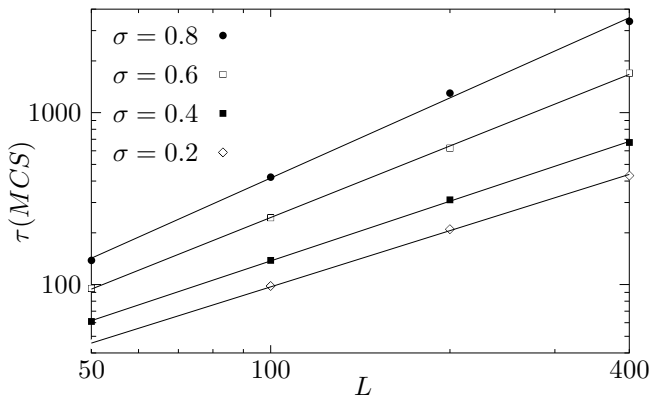
FIG. 5: Integrated autocorrelation time \tau vs. lattice size L for q = 7 and \sigma = 0.2, 0.4, 0.6, 0.8 . Dynamic exponents computed from a fit to L^z are z = 1.09(1), 1.15(1), 1.38(1), 1.55(1) respectively.
