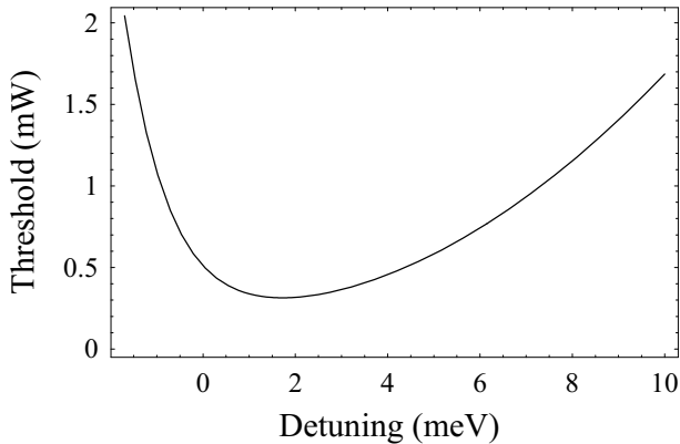
FIG. 2: Variations of the bistability threshold in milliwatts versus the cavity-exciton detuning. The parameters are the same as in Fig. 1.
