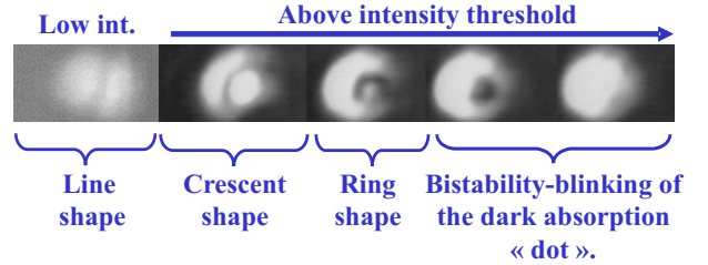
FIG. 5: Near-field images of the reflected beam. The laser wavelength is 831.69 nm, resonant with the lower polariton at \delta = 0.3 meV. The first image is taken at very low excitation intensity (0.2 mW). All the other images are taken at 2 mW, for different positions of the excitation spot on the sample. The last two images are obtained for the same position ; we observed a blinking between these two states, due to mechanical vibrations.
