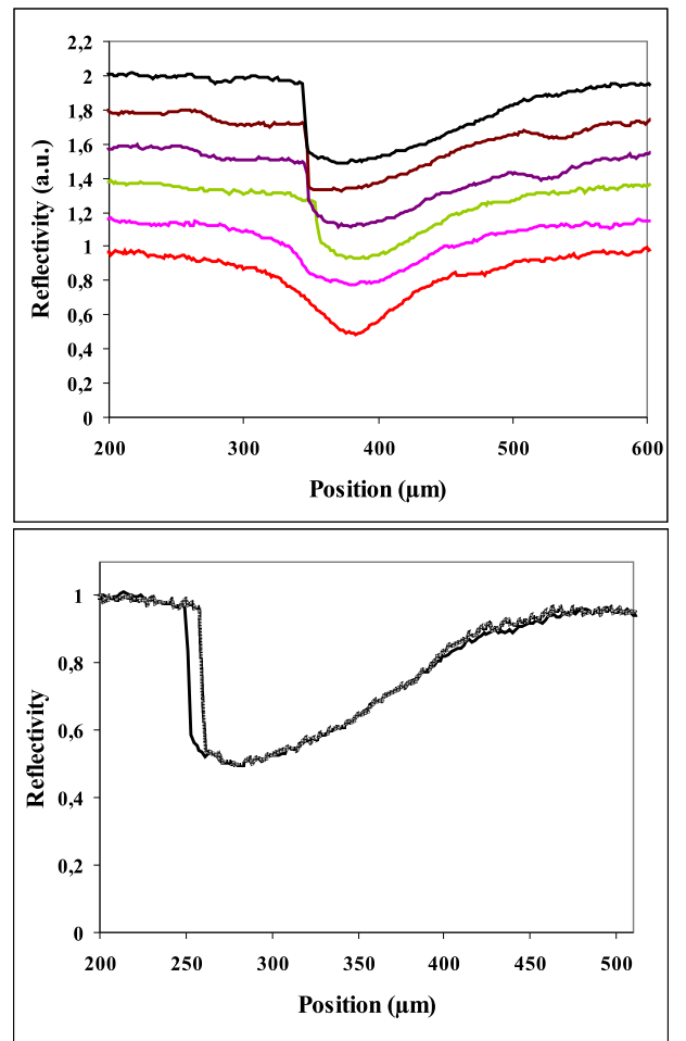
FIG. 7: Upper figure: reflected intensities (in arbitrary units) as a function of the spot position on the sample (the origin of the axis is arbitrary), for several values of the input power I^{in} : 1, 2, 3, 4, 5 and 6 mW. The laser wavelength is 831.32 nm, resonant with the lower polariton at \delta = 1.5 \text{ meV} . Bistability appears at I^{in}=2.8 \text{ mW} . Lower figure: hysteresis cycle for the curve I^{in} = 6 \text{ mW} . The two curves correspond to the two directions for the scan of the spot position on the sample.
