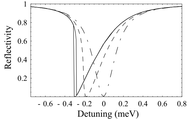
FIG. 3: Reflectivity spectra as a function of the cavity-exciton detuning, for I^{in} near zero (dash-dotted line), I^{in}=0.5 mW (dashed line) and I^{in}=1 mW (solid line). The laser energy is E_L = E_{exc} - \Omega_R/2 , equal to the lower polariton energy at zero cavity-exciton detuning in the absence of nonlinear effects. The other parameters are the same as in Fig. 1. The reflectivity resonance is indeed at \delta = 0 in the low intensity case but it is shifted at higher intensity. For the highest intensity, a hysteresis cycle appears when scanning the spot position in the two directions.
