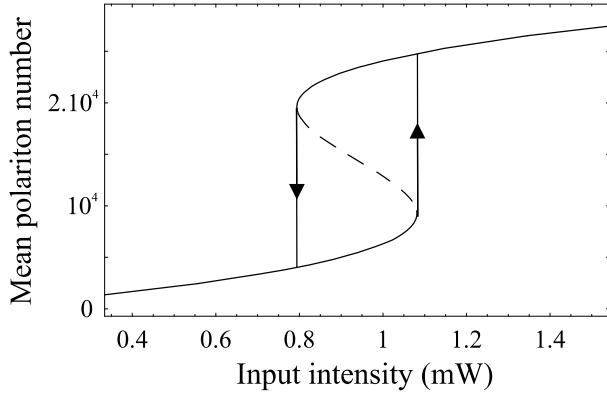
FIG. 1: Intensity of the polariton field (i.e. the mean number of polaritons n_p ) versus the input power I^{in} in milliwatts. The nonlinear coefficient is V_0=4.5 \cdot 10^{-5} meV (corresponding to a spot of 50 \mu\text{m} in diameter). The cavity and exciton linewidths are \gamma_a=0.12 meV and \gamma_b=0.075 meV and the polariton linewidth is taken as equal to \gamma_p = C_0^2\gamma_a + X_0^2\gamma_b (see text). The cavity-exciton detuning is \delta=0 . The laser detuning is \delta_p=2.5 \gamma_p . In the bistable region, the dotted line is the unstable branch. The arrows indicate the hysteresis cycle obtained by scanning the input power in both directions.
