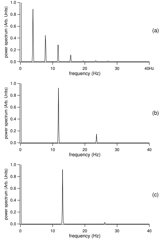
Fig. 27. Power spectra of the atomic cloud location Z in the unstable zone. Parameters are the same as in Fig.24.
