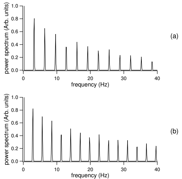
Fig. 29. Power spectra of the atomic cloud location Z in the unstable zone. Parameters are the same as in Fig.24.
