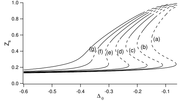
Fig. 16. Evolution as a function of the detuning of the stationary solution Z_s of equations 1 for different values of n_0 and a smaller atomic density than in Fig. 11. The full (resp. dashed) line corresponds to a stable (resp. unstable) solution. In (a), n_0 = 2 \times 10^8 ; in (b) n_0 = 4 \times 10^8 ; in (c), n_0 = 6 \times 10^8 ; in (d), n_0 = 8 \times 10^8 ; in (e), n_0 = 1 \times 10^9 ; in (f), n_0 = 1.2 \times 10^9 ; in (g), n_0 = 1.4 \times 10^9 . Other parameters correspond to the set #1 of Table 2, with \rho = 1 \times 10^{10} \text{ cm}^{-3} .
