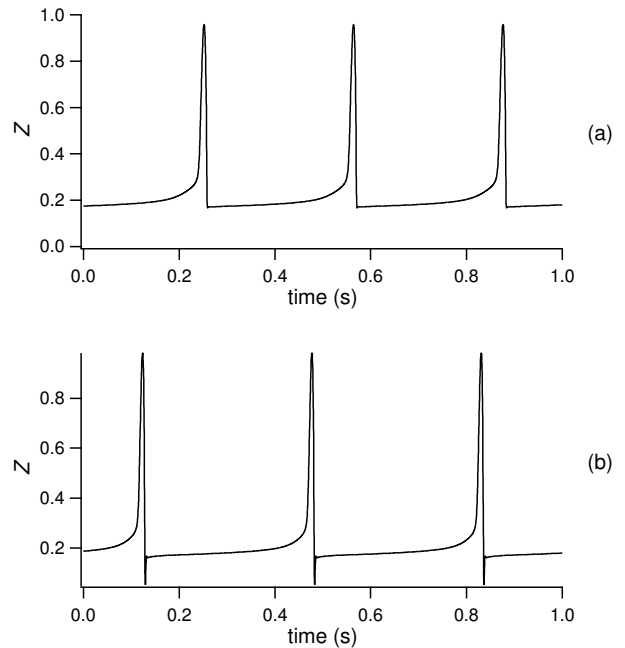
Fig. 28. Time evolution of the atomic cloud location Z (left) and population N (right) in the unstable zone. In (a), \Delta_0 = -0.36 ; in (b), \Delta_0 = -0.35 .
