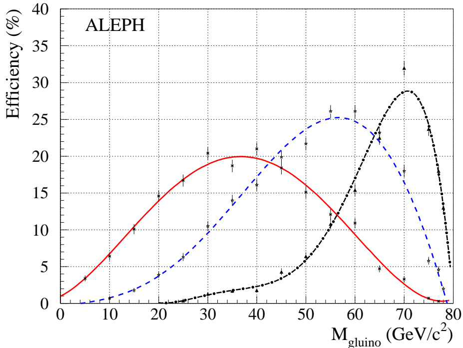
Figure 11: The three parametrized selection efficiencies for m_{\tilde{t}} = 80 \text{ GeV}/c^2 (full curve, large \Delta M selection; dashed curve, intermediate \Delta M selection; and dot-dashed curve, small \Delta M selection) as a function of m_{\tilde{g}} . The dots with error bars show the actual efficiencies obtained from the individual simulated samples.
