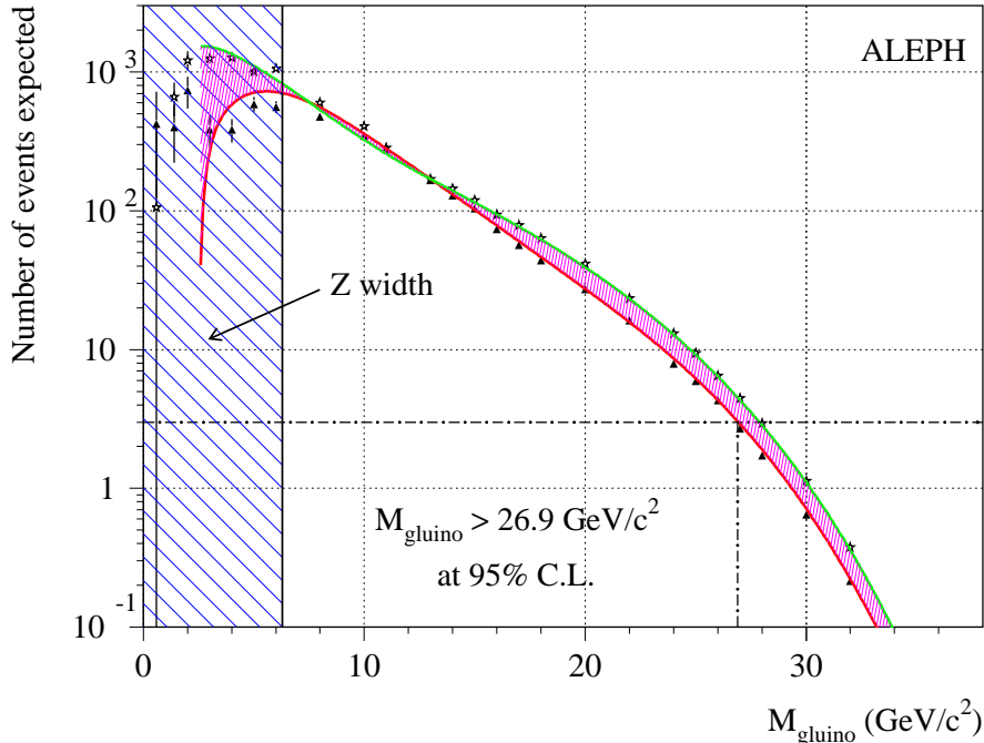
Figure 6: The number of q\bar{q}\tilde{g}\tilde{g} events expected to be selected in the LEP 1 data by the neutral and charged R-hadron searches, as a function of the gluino mass, for P_{\tilde{g}\tilde{g}} varying between 0 and 1 (shaded area). The markers with error bars (triangles for P_{\tilde{g}\tilde{g}} = 1 , stars for P_{\tilde{g}\tilde{g}} = 0 ) show the individual values obtained from each of the simulated signal samples. Also shown is the region excluded by the Z lineshape measurement (hatched region), and the lower limit on the gluino-LSP mass (dot-dashed lines).
