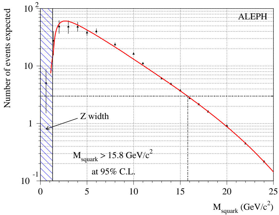
Figure 7: The number of q\bar{q}q\bar{q} events expected to be selected in the LEP 1 data as a function of the squark mass (full curve). The triangles with error bars show the individual values obtained from each of the simulated signal samples. Also shown is the region excluded by the Z lineshape measurement (hatched region), and the lower limit on the squark-LSP mass (dot-dashed lines).
