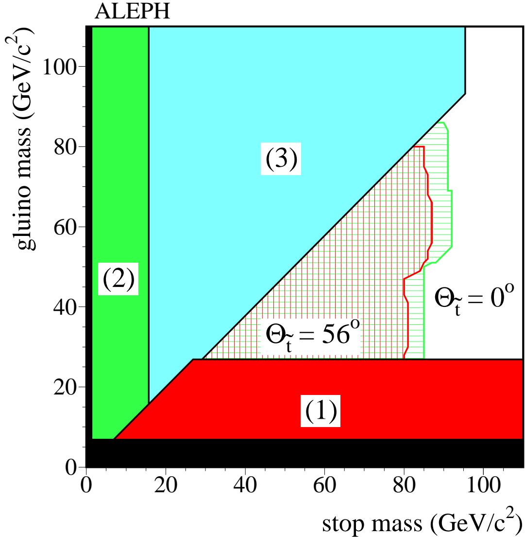
Figure 13: The 95% C.L. excluded regions in the plane (m_{\tilde{t}}, m_{\tilde{g}}) from the combination of all searches presented in this paper. The black area at very small gluino and squark masses is excluded by the precise measurement of the Z lineshape; Regions (1), (2) and (3) are excluded by the search for e^+e^- \rightarrow q\bar{q}\tilde{g}\tilde{g} at LEP 1, for e^+e^- \rightarrow q\bar{q}\tilde{q}\tilde{q} at LEP 1, and for heavy stable charged particles from \tilde{q}\tilde{q} production at LEP 2, respectively. The hatched areas are excluded by the acoplanar jet with missing energy search at LEP 2.
