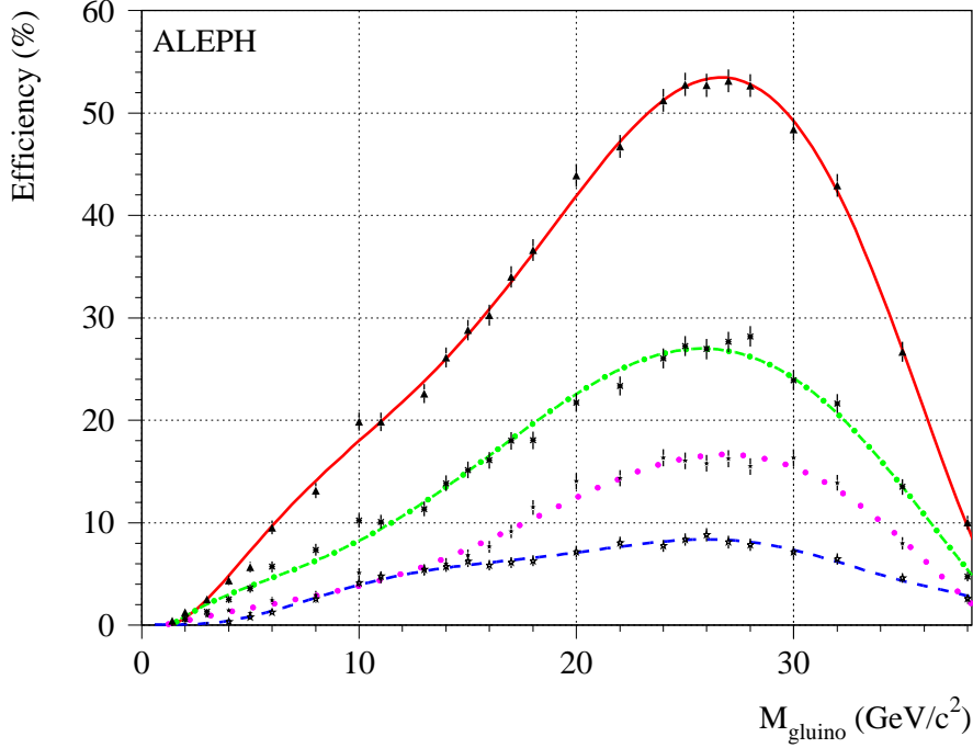
Figure 5: The q\bar{q}g\bar{g} selection efficiency as a function of the gluino mass, when P_{g\bar{g}} = 0\% , for the q\bar{q}R^0R^0 final state (dashed curve), the q\bar{q}R^\pm R^0 final state (dot-dashed curve), the q\bar{q}R^\pm R^\pm final state (dotted curve), and the sum of the three (full curve). The markers with error bars indicate the efficiencies obtained with each of the simulated samples, and the curves are obtained with a polynomial fit through these points.
