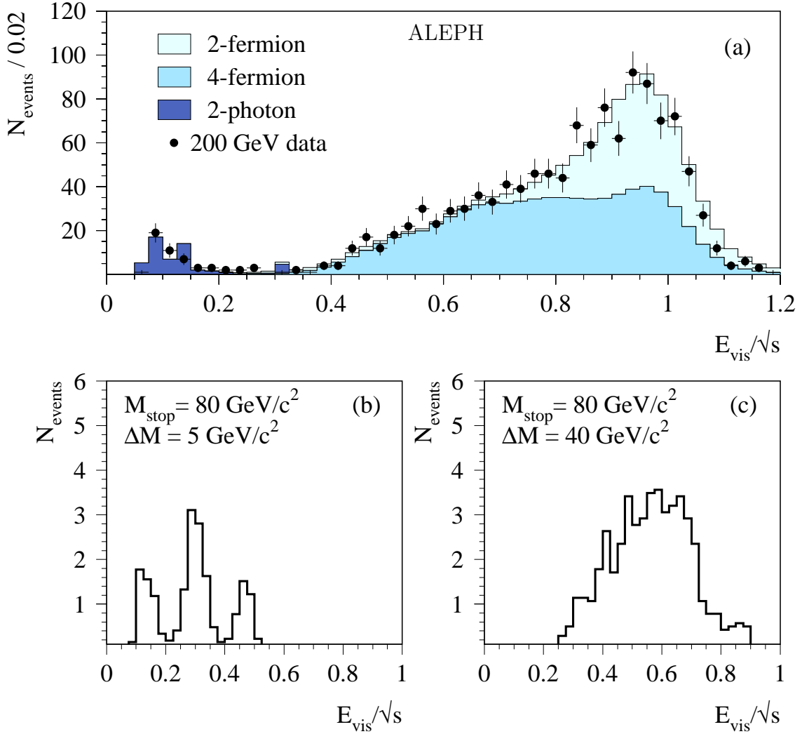
Figure 10: Distributions of the visible energy observed in the data at \sqrt{s} = 200 \text{ GeV} (dots with error bars) and expected from various background sources (shaded histograms), after the preselection cuts (a). The lower two plots show the expected distributions for the signal, with \Delta M = 5 \text{ GeV}/c^2 (b) and 40 \text{ GeV}/c^2 (c). For small \Delta M , the R-hadron composition is clearly visible: double-charged-R-hadrons events have largest visible energy, and double-neutral-R-hadrons events have smallest visible energy. For large \Delta M , the three peaks are merged because of the broader visible energy distributions.
