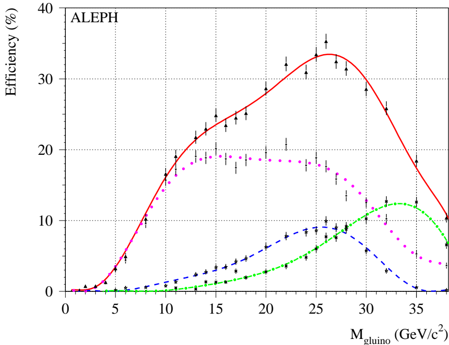
Figure 2: The q\bar{q}\tilde{g}\tilde{g} selection efficiency as a function of the gluino mass, for the H\nu\bar{\nu} selection (dashed curve), the additional efficiency of the large-mass selection (dot-dashed curve), the additional efficiency of the small-mass selection (dotted curve), and the sum of the three (full curve). The markers with error bars indicate the efficiencies obtained with each of the simulated samples, and the curves are obtained with a polynomial fit through these points.
