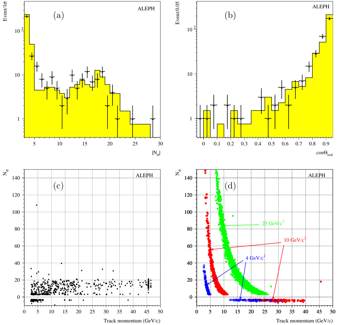
Figure 4: Distributions of (a) |N_\sigma| , the number of standard deviations with respect to the expected dE/dx for the most-likely light-particle hypothesis; and (b) the cosine of the isolation angle, for the heavy-stable-charged-particle track candidates after the preselection, in the data (triangles with error bars) and the background simulation (histogram). Distributions of N_\sigma as a function of the charged particle momentum (c) in the data and (d) in the signal simulation with m_{\tilde{g}} = 4, 10 and 25 \text{ GeV}/c^2 .
