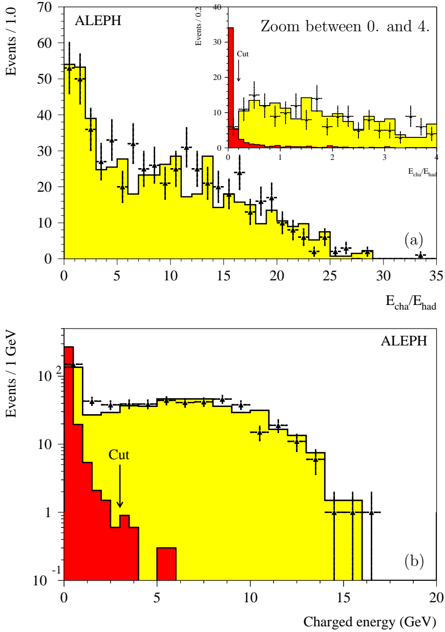
Figure 3: Distributions of (a) the ratio of the “R-hadron jet” charged energy to its neutral hadronic energy; and (b) the charged energy in a 35^\circ cone around the missing momentum, before the corresponding cuts are applied, for the data (triangles with error bars), the background simulation (light-shaded histogram) and the signal with m_{\tilde{g}} = 10 \text{ GeV}/c^2 (dark-shaded histogram, arbitrary normalization).
