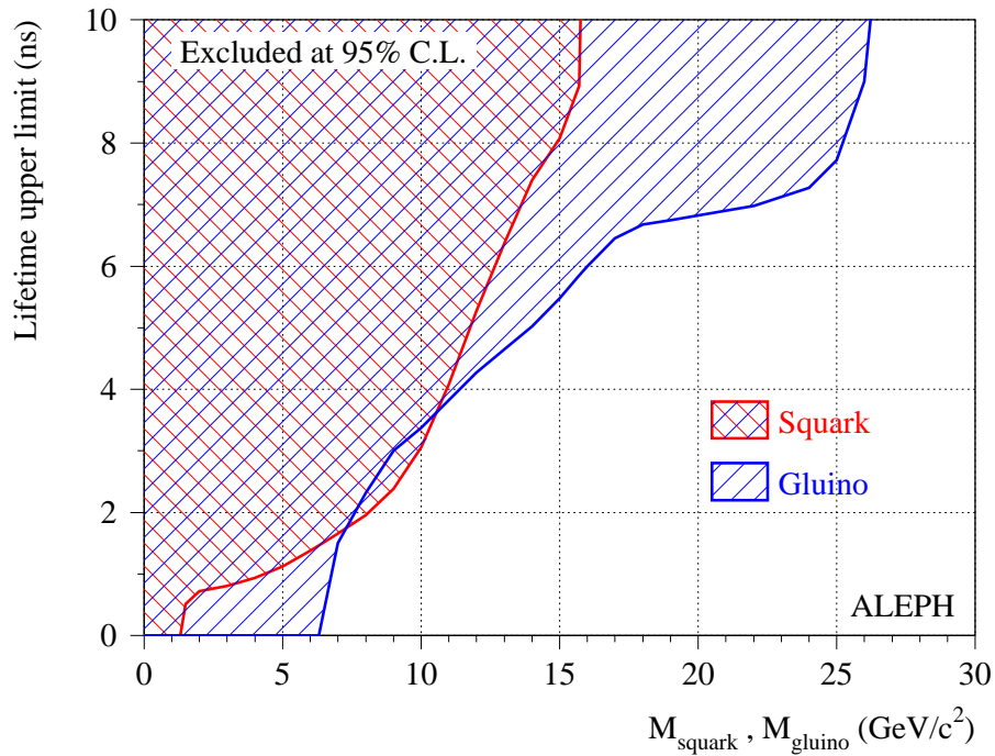
Figure 8: The upper limit on the squark and gluino lifetimes as a function of their mass (full curve). The hatched areas are excluded at more than 95% C.L.
