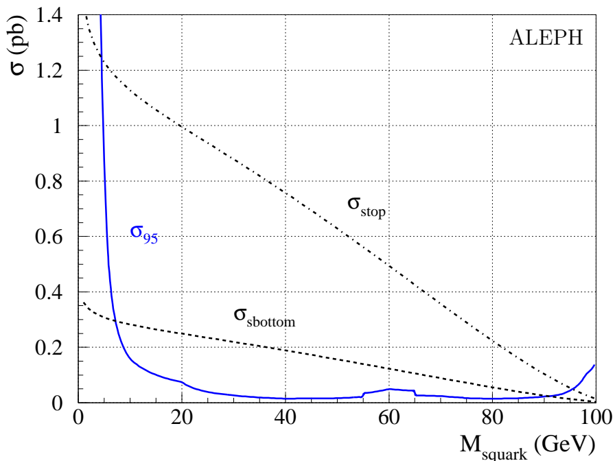
Figure 9: The production cross sections for e^+e^- \rightarrow \tilde{t}\tilde{t}^* and \tilde{b}\tilde{b}^* at \sqrt{s} = 209 GeV, as a function of the squark mass. Also shown is the observed 95% C.L. upper limit on the cross section, derived from the stable stop search of Ref. [3].
