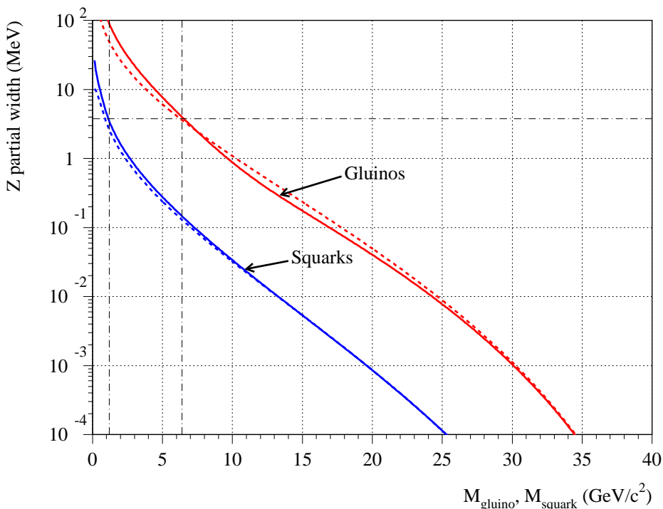
Figure 1: The Z \rightarrow q\bar{q}\tilde{g}\tilde{g} and Z \rightarrow q\bar{q}\tilde{q}\tilde{q} partial widths as a function of the squark and the gluino mass, computed at the leading order (dashed curves) and resummed at the next-to-leading order (full curves). Also shown are the corresponding 95% C.L. lower limits on the squark and gluino masses when the contribution to the Z width exceeds 3.9 MeV (Ref. [17] and Section 4).
