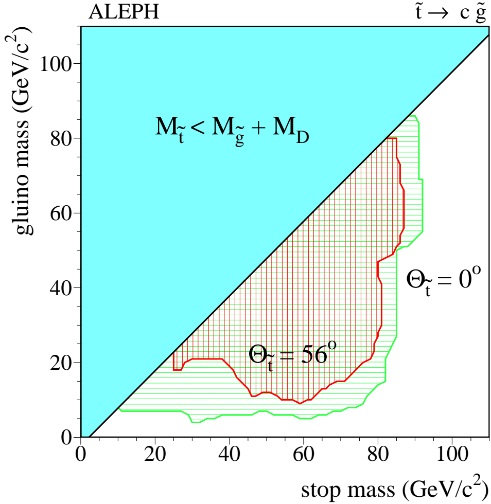
Figure 12: The 95% C.L. excluded regions in the plane (m_{\tilde{t}}, m_{\tilde{g}}) from the acoplanar jet search at LEP 2, for maximal (horizontal hatching) and minimal (cross hatching) stop coupling to the Z. The shaded area corresponds to a stable stop and is not accessible to this search.
