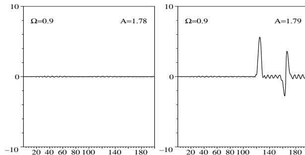
Figure 2: Representation of u_n(t) as a function of time for n = 60 in the case \Omega = 0.90 for two amplitudes.
