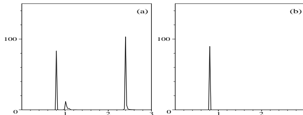
Figure 1: Spectra of the particle 50 submitted to, (a) harmonic boundary driving at frequency 0.8 and amplitude 2 and to, (b) breather boundary driving at frequency 0.8.
