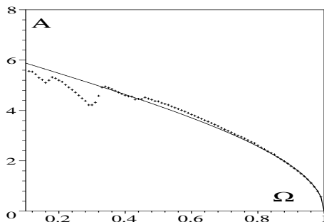
Figure 4: Bifurcation diagram in the (A, \Omega) plane. The solid line is the threshold expression (10). The crosses indicate the lowest value of A for which non-linear supratransmission is seen on numerical simulations.
