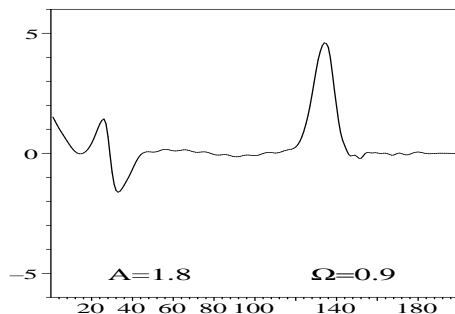
Figure 3: Plot of u_n(t) as a function of n at t = 120 .
