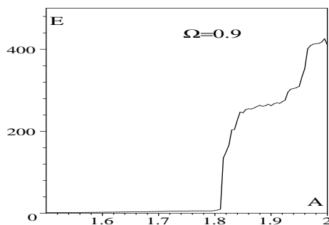
Figure 12: Energy in the Klein-Gordon chain (24).
