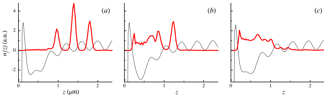
FIG. 6: Results of the numerical simulation of the atomic lift: integrated spatial density along x and y as a function of z (thick curve), at three evolution times: (a) t = 5.8 ms; (b) t = 13.3 ms; (c) t = 22.3 ms. The potential is also represented (thin curve).
