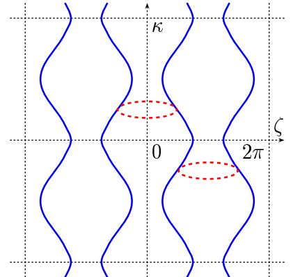
Figure 2: The phase space picture
