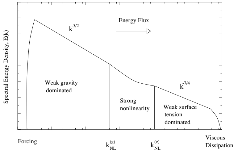
FIG. 1: Schematic representation of the different scaling regimes in the surface wave problem. The width of the window of fully nonlinear turbulence depends on the energy flux input at the forcing scale.
