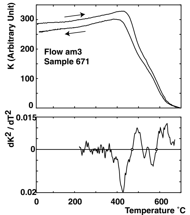
Figure 4. Example of thermal variation of weak-field magnetic susceptibility K (measured in an induction field B equal to 100 \mu\text{T} ) against temperature T ( ^{\circ}\text{C} ) showing a good reversibility and second derivative of the smoothed data of the heating curve. The mean Curie temperature is defined when the second derivative increases to zero (Prévoit et al. 1983).
