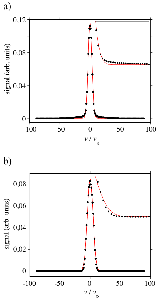
FIG. 9: Numerically recorded velocity distributions with fits to simple Gaussians. For a, the modulation depth of the optical potential was U_0 = 78 E_R . For b, it was U_0 = 235 E_R . The insets show magnifications of portions of the wings of the distributions.
