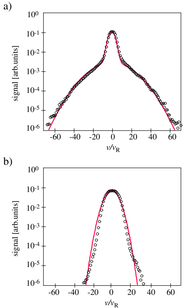
FIG. 11: Numerically computed velocity distribution for a) U_0 = 78E_R and b) U_0 = 293E_R together with fits to Double Gaussians.
