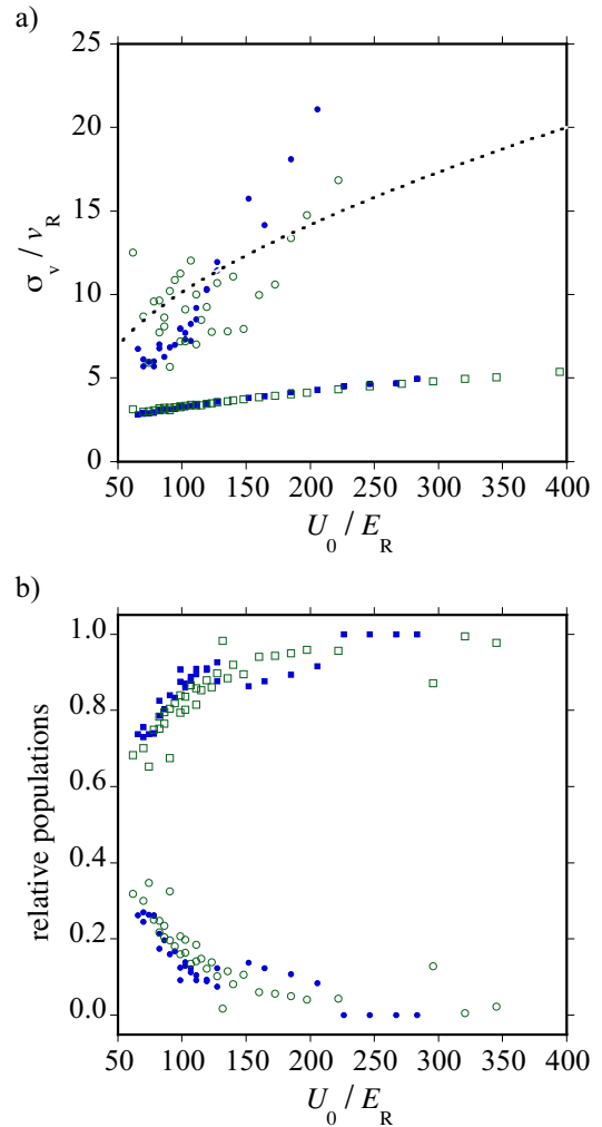
FIG. 7: a) The widths of the two Gaussians as obtained from a fit of the data to double Gaussians, as a function of modulation depth of the potential. The dashed line shows the modulation depth in units of velocity. b) The relative population of the two modes of the population, obtained from the areas under the two Gaussians. For both a) and b), filled symbols correspond to data taken with 50 ms equilibration time and open symbols to 25 ms. Circles are ‘temperatures’ and relative population of the ‘hot mode’, and square to the ‘cold mode’.
