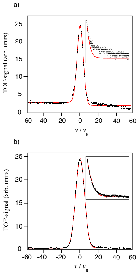
FIG. 3: Experimentally recorded velocity distributions with fits to simple Gaussians. This data is recorded with an equilibration time of 25 ms. For a the modulation depth of the optical potential was U_0 = 78E_R and the shown data is an average of 20 TOF measurements. For b the corresponding facts were U_0 = 285E_R and an average of 5 TOF measurements. The insets show magnifications of portions of the wings of the distributions.
