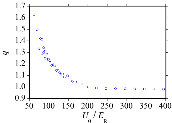
FIG. 6: The fitted Tsallis q -parameter as a function of modulation depth of the potential for 25 ms equilibration time.
