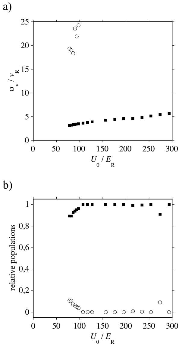
FIG. 12: a) Widths of the two Gaussians (cold mode: filled circles, hot mode: open circles) as obtained from a fit of the numerical data to Double Gaussians, as a function of modulation depth of the potential. b) The relative population of the two modes of the velocity distributions, obtained from the areas under the two Gaussians. The cold mode (filled circles in a) corresponds to the large fraction whereas the hot mode (open squares) corresponds to the small fraction.
