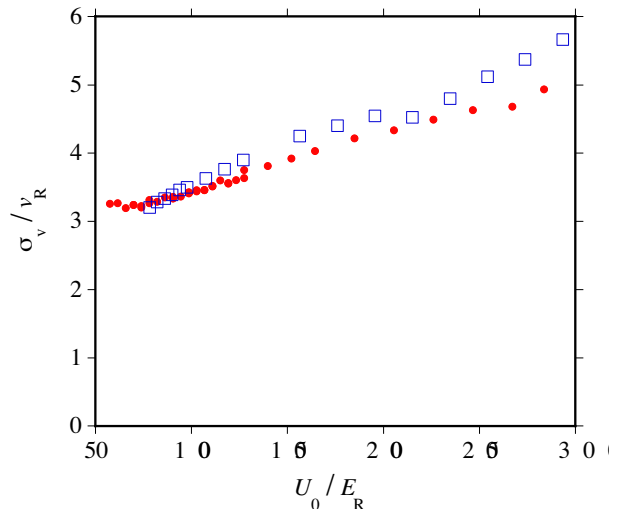
FIG. 2: The rms width ( \sigma_v ) of the measured velocity distributions (filled circles) as a function of the modulation depth of the potential. Also shown is numerically simulated data (open squares) in the same range (c.f. chapter IV).
