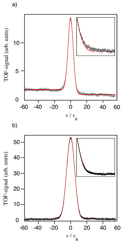
FIG. 4: Experimentally recorded velocity distributions with fits to simple Gaussians. This data is recorded with an equilibration time of 50 ms. For a the modulation depth of the optical potential was U_0 = 78E_R and the shown data is an average of 20 TOF measurements. For b the corresponding facts were U_0 = 285E_R and an average of 5 TOF measurements. The insets show magnifications of portions of the wings of the distributions.
