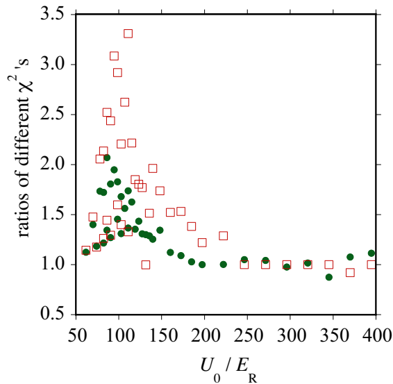
FIG. 5: Comparisons between different fits of the measured distribution for 25 ms equilibration time shown as ratios between unnormalized values of \chi^2 as a function of modulation depth of the potential. The circles are \chi_{1\text{Gauss}}^2/\chi_{\text{Tsallis}}^2 and the squares are \chi_{1\text{Gauss}}^2/\chi_{2\text{Gauss}}^2 .
