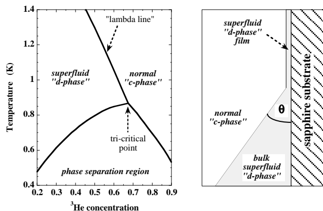
FIG. 1. The phase diagram of ^3\text{He} - ^4\text{He} mixtures (left graph). On the right, a schematic view of the contact angle \theta . There is a superfluid film of ^4\text{He} rich “d-phase” between the substrate and the c-phase. Its thickness being finite, \theta is non-zero.
