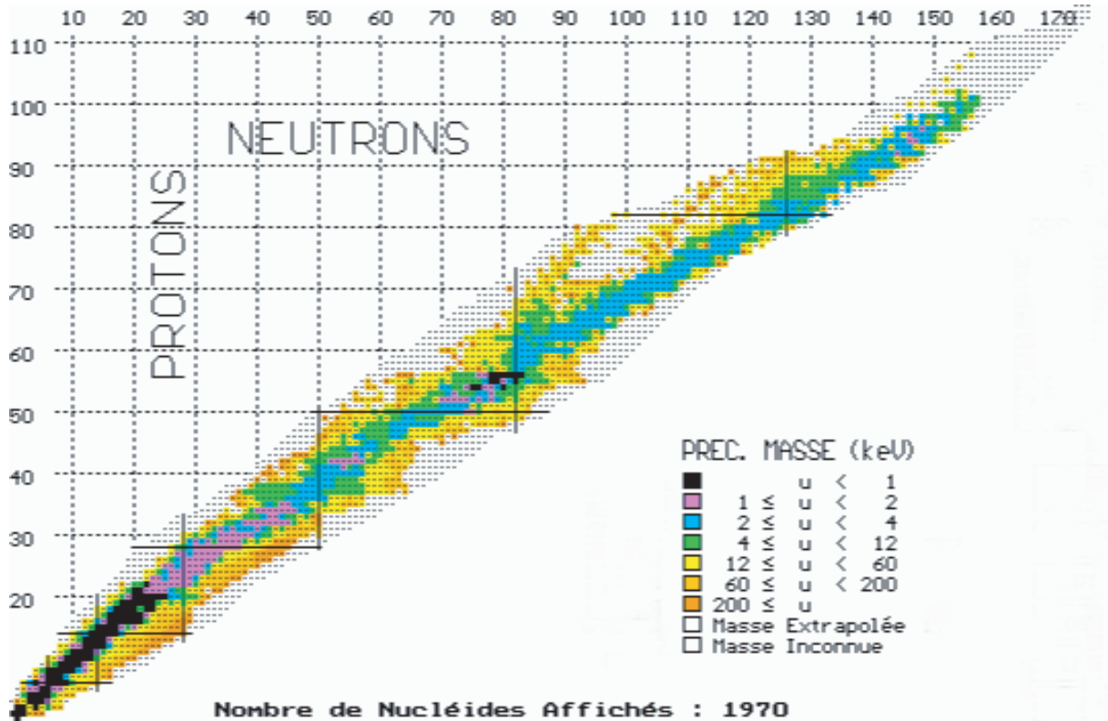
Figure 1: Chart of nuclides for the precision on masses. Only the known masses are colored, exhibiting crudely the narrowness of the valley of our knowledge in this immense landscape. Would these 1970 known masses been scattered around in the (N, Z) plane, our understanding of the nucleus would have been completely changed.
