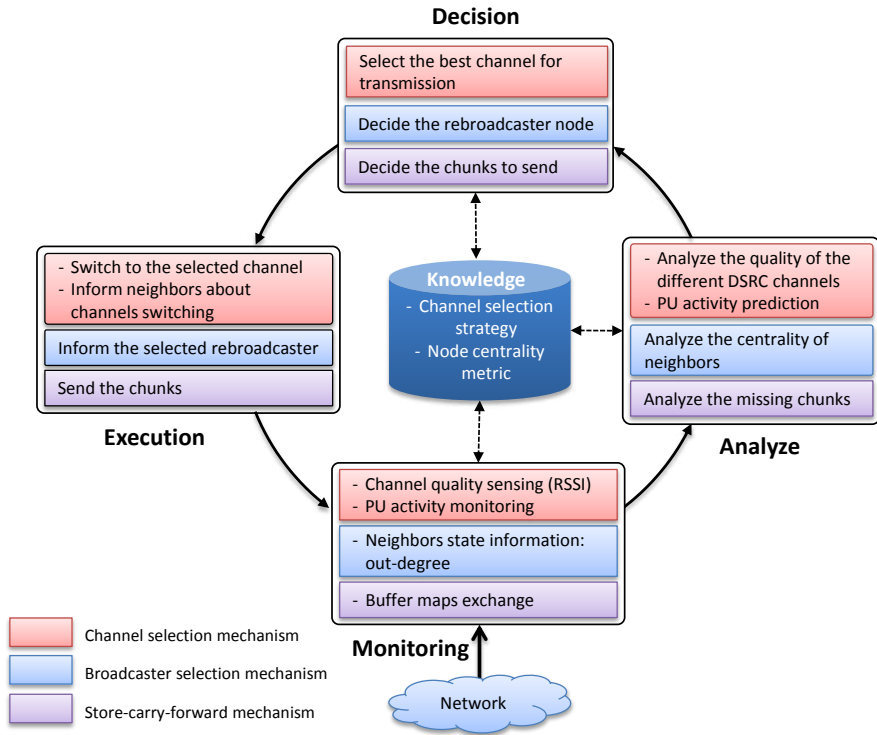
Figure 4: ViCoV architecture
