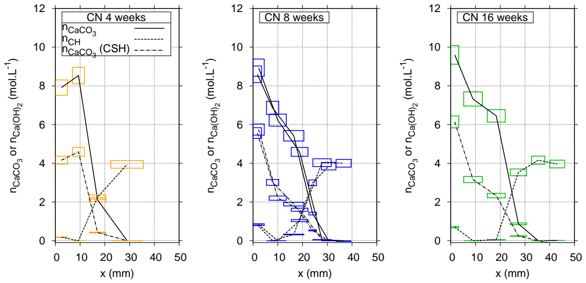
Figure 13: Carbonation profiles assessed by TGA-MS. Illustration of contents of CH and \overline{\text{C}}\overline{\text{C}} (for \overline{\text{C}}\overline{\text{C}} , total content and content only related to C-S-H carbonation are illustrated) after 4, 8 et 16 weeks of exposure to \text{CO}_2 . Case of CN paste. For the case of 8 weeks of exposure, the profiles for two different specimens are shown.
