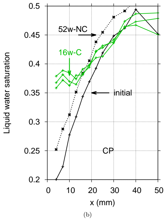
Figure 23: Water saturation profile obtained by GRAM for both CN and CP at the initial state, after 8 and 16 weeks of carbonation (8w-C and 16w-C, resp.). The profiles for the control specimens are illustrated (16 weeks for CN and 52 weeks for CP).
