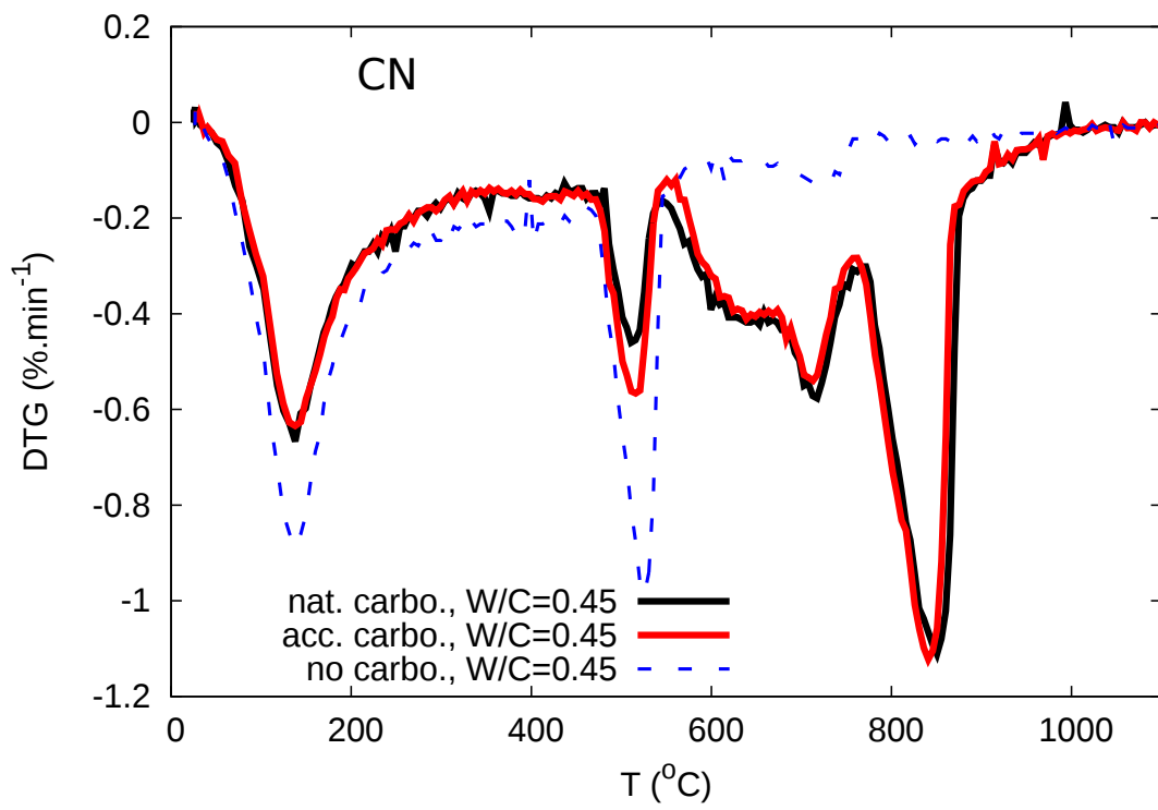
Figure 11: Comparison of DTG diagrams between non-carbonated and carbonated CN (10% CO 2 or natural carbonation).
