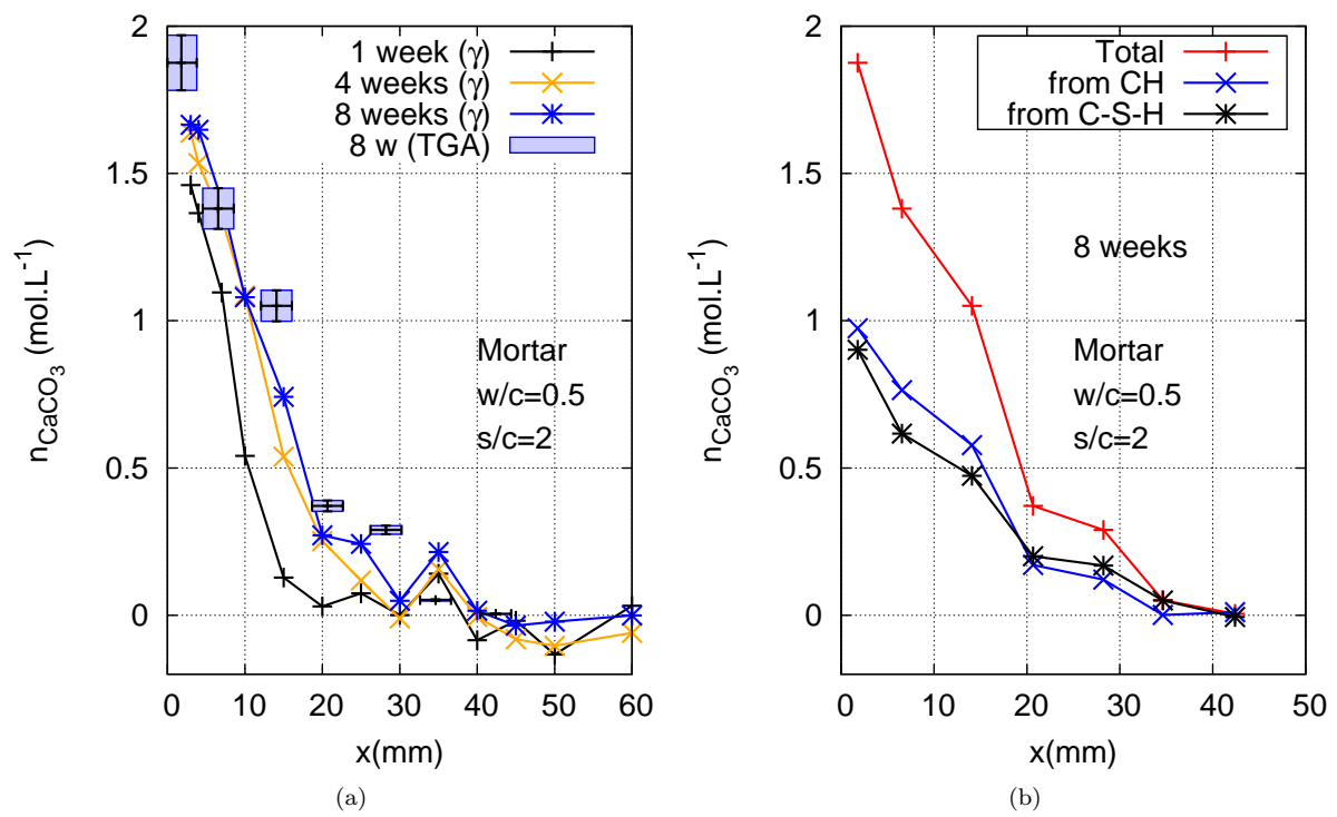
Figure 17: (a) Content of the \text{CO}_2 fixed to the cement matrix as \overline{\text{CC}} are represented for the studied mortar (CEM I cement, w/c=0.5 and s/c=2 ). TGA results are represented by coloured boxes while GRAM are represented as coloured lines. (b) Quantification of total \overline{\text{CC}} (red) and balance between n_{\text{CC}}^{\text{CH}} (blue) or n_{\text{CC}}^{\text{CSH}} (black) after 8 weeks of carbonation for the mortar
